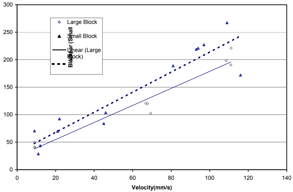
Figure 4.5 Shear Strength VS. Speed Rubble Thickness - 0.4 m, Zero Consolidation
