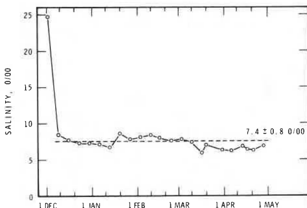
Fig. 7. Variation of salinity with time for 2.5 cm sections of ice at a depth between 40 and 42.5 cm. Broken line indicates "stable" salinity or average of all the salinities except the initial high value at this level.
