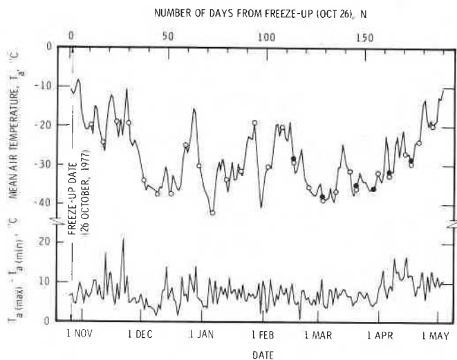
Fig. 1. Variation of daily mean air temperature \frac{1}{2}(T_a(\max) + T_a(\min)) and corresponding difference between maximum and minimum temperatures during winter of 1977-78 at Pond Inlet. Open and solid circles indicate dates on which ice cores were taken and ice temperatures measured, respectively.
