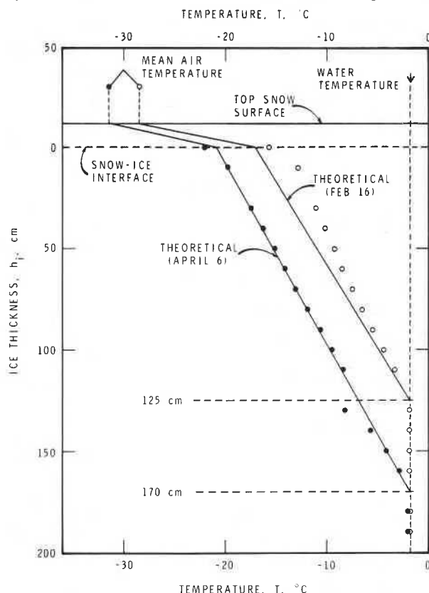
Fig. 3. Comparison between measured and theoretical temperature distributions in ice sheet for two days in 1978. Theoretical calculations are based on mean air temperatures for days shown, water temperature of -1.8^\circ\text{C} , snow depth of 11.4 cm and ice thickness estimated from temperature distributions.
