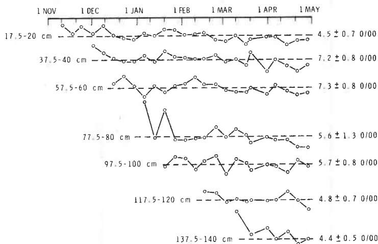
Fig. 8. Attainment and retention of "stable" brine content at a given depth, during winter of 1977-78, for various depths at intervals of 20 cm as shown.
