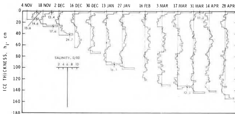
Fig. 6. Salinity profile in ice of Eclipse Sound at intervals of two weeks during winter of 1977-78. Scale for salinity is shown in insert. Vertical solid lines represent a value of 6‰ and are given as a reference.
