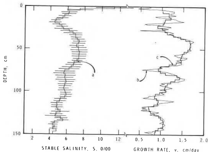
Fig. 9. Curve a shows variation of "stable" salinity with depth at intervals of 2.5 cm. Horizontal bars represent standard deviations. Curve b gives dependence of growth rate on depth, calculated on basis of air temperatures. Curve c represents running mean of calculated growth rate for an interval of \pm 5 cm for every 2.5 cm segment of ice.
