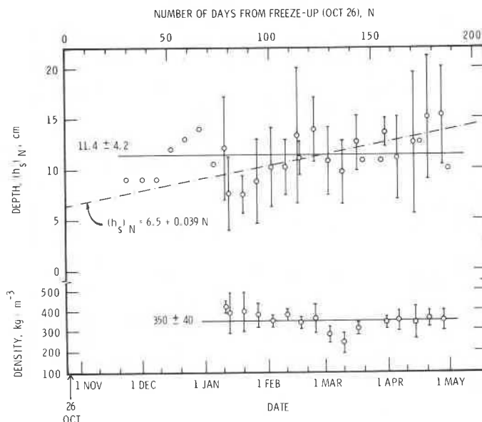
Fig. 2. Variation of snow depth and density during winter of 1977-78. Isolated circles for snow depth indicate single measurements, and circles with standard deviation bars describe the mean of six to eight measurements. Each data point for snow density indicates the mean of six measurements.
