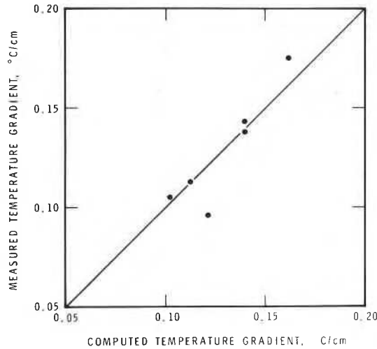
Fig. 4. Comparison between calculated and measured temperature gradients in an ice sheet for six measurements carried out during February–April 1978, in Eclipse Sound.
