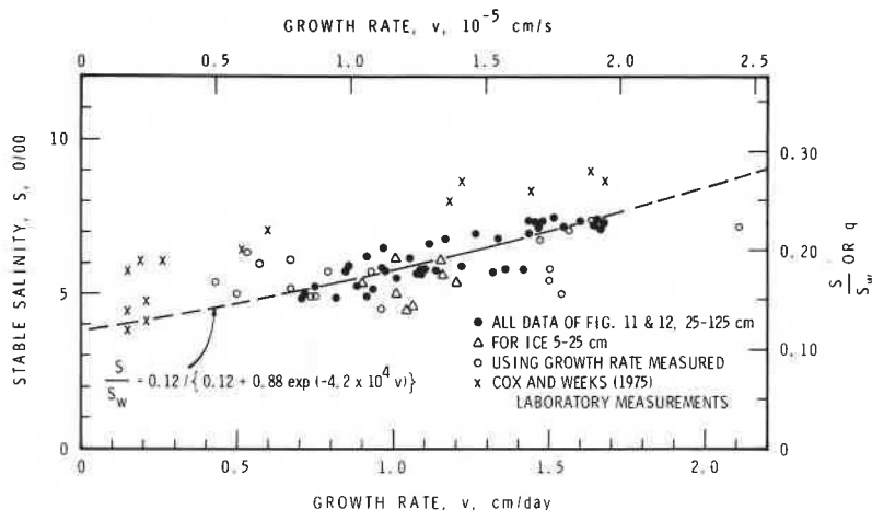
Fig. 13. "Stable" salinity versus growth rate.
