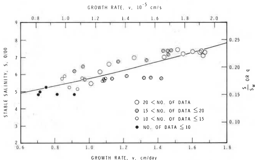
Fig. 11. Plot of "stable" salinity S of each 2.5 cm segment of curve a versus corresponding growth rate v of curve b of Figure 9 for columnar-grained ice at depths between 25 and 125 cm. Number of segment salinities available for determining each S value is shown. Solid line represents Equation (18) for \delta/D = 4.2 \times 10^{-4} s/cm and q_0 = 0.12 .
