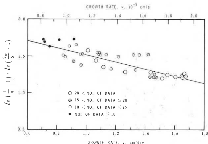
Fig. 12. Plot of \ln(1/q - 1) or \ln(S_w/S - 1) versus growth rate for columnar-grained ice observed for depths between 25 and 125 cm. Number of segment salinities available for determining each S value is shown. Solid line represents the least-square fit of Equation (20) to all the data, giving \delta/D = 4.2 \times 10^4 s/cm and q_0 or S_0/S_w = 0.12 .
