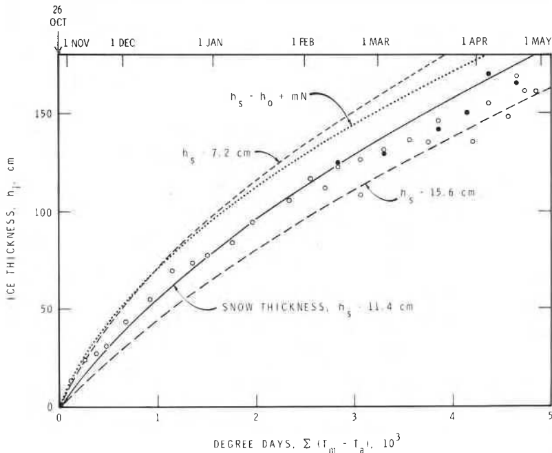
Fig. 5. Growth of ice in Eclipse Sound during winter of 1977–78. Open circles represent measured ice thicknesses. Solid circles give thicknesses estimated from measured temperature distributions. Solid and broken lines are calculations (Equation (11)) for snow thicknesses of 11.4 \pm 4.2 cm. Dotted line is based on Equation (17) for variable snow thicknesses.
