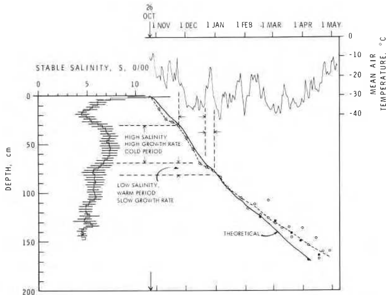
Fig. 10. Composite diagram of "stable" salinity profile, variation of daily mean air temperature with time during winter of 1977-78, and growth history of the ice. Open circles are measured ice thicknesses. Solid circles give thicknesses estimated from measured temperature distributions. Growth curve (broken line) is an "eye-fit"; solid curve is based on theory. High salinity is related to high growth that corresponds to colder periods. Warmer days slowed the growth of ice, resulting in lower salinity.
