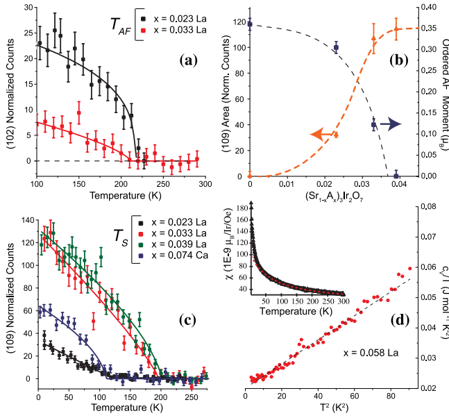
FIG. 2 (color online). (a) Background subtracted magnetic order parameter measurements for La-doped Sr-327. Data were collected at the \mathbf{Q} = (1, 0, 2) position and normalized to a sample-dependent scale factor. (b) AF-ordered moment and relative weight of forbidden structural peak (1,0,9) (representative of T_S for La-doped Sr-327). Data for x = 0 were taken from Ref. [17]. (c) Background subtracted neutron scattering data showing select T_S order parameters at the (1,0,9) wave vector. Intensity of the scattering has been normalized via a sample-dependent scale factor. (d) Heat capacity c_v(T) data for x = 0.058 La. Dashed line is a fit to the form c_v(T) = \gamma T + \beta T^3 with \gamma = 19.88 \pm 0.30 (mJ mole ^{-1} K ^{-2} ) and \beta = 0.409 \pm 0.007 (mJ mole ^{-1} K ^{-4} ). Inset shows \chi(T) for this same sample with H = 20 kOe \parallel ab plane with dotted line denoting the Curie-Weiss fit discussed in the text.
