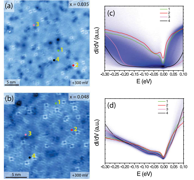
FIG. 3 (color online). STM topography of La-doped Sr-327 at 300 mV bias for (a) insulating x = 0.035 and (b) metallic x = 0.048 samples. dI/dV spectra obtained on a grid in each topograph are plotted in panels (c) for x = 0.035 and (d) for x = 0.048 . Representative numbered points are highlighted in each map and the corresponding dI/dV spectra are emphasized as solid lines in spectral histograms. Fully gapped and gapless spectra are observed in the x = 0.035 sample, while a homogeneous, gapless state appears across spectra in x = 0.048 .
