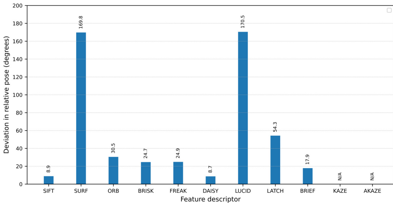
(b) Deviation in relative pose vs the type of features
