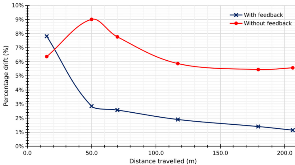
Fig. 12. Percentage drift versus distance travelled.
