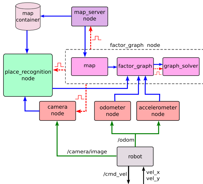
Fig. 6. The schematic of the factor graph-based localization system.
