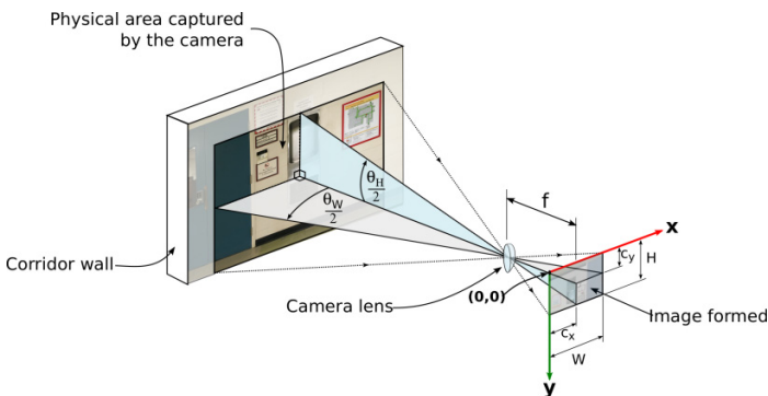
Fig. 4. Pin hole model of the camera. The coordinate system of the formed image has the x -axis (in red) pointing right and the y -axis pointing down with the origin located at the top-left corner of the image.
