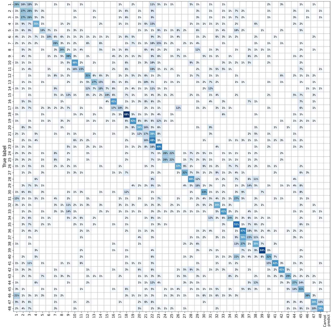
(a) Confusion matrix before distance thresholding
