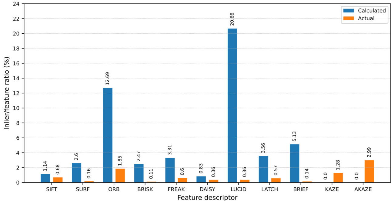
(a) Calculated and actual inlier/feature ratio vs the type of features
