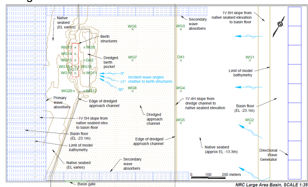
Figure 1 - Physical model basin layout (Baker et al. , 2019).
