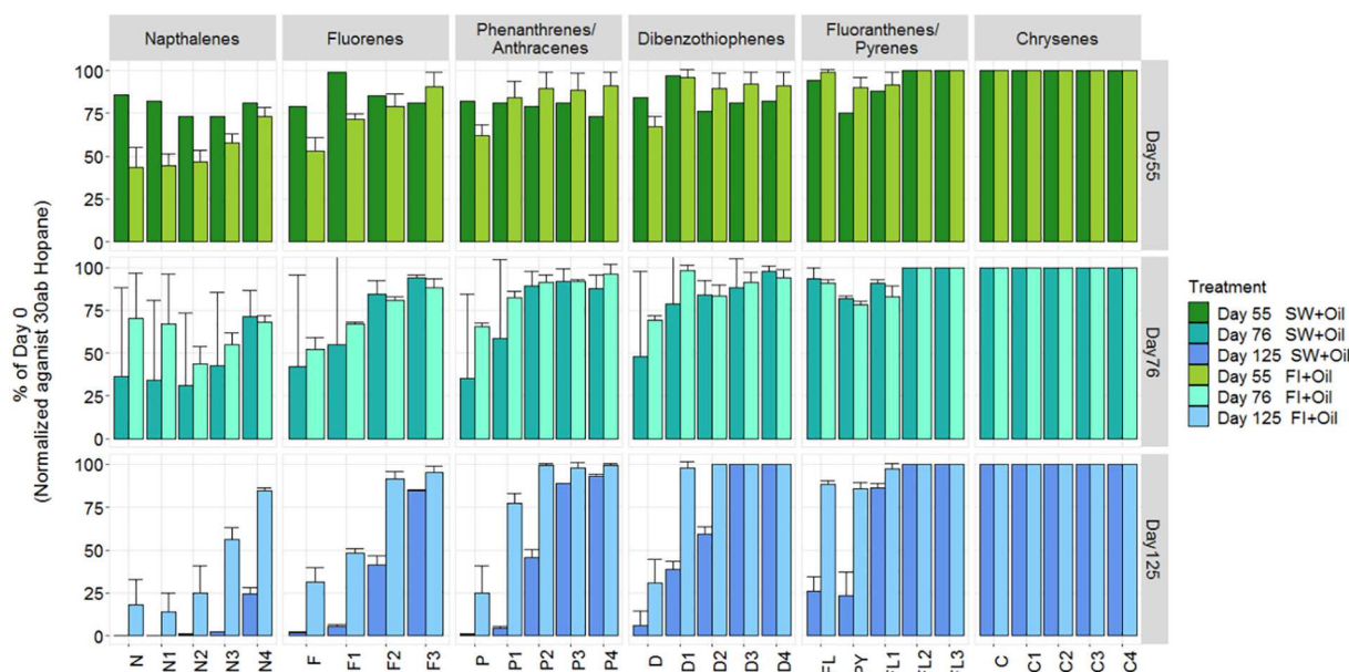
Fig. 2. Degradation of target PAHs in seawater with frazil ice (FI+oil), and without frazil ice (SW+oil). The losses are given as percentages of day 0, after normalization against 30ab Hopane. Different colours represent the sampling days from day 0 to day 125.
