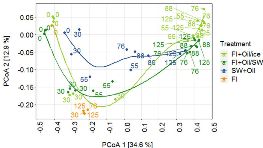
Fig. 5. Change in microbial community structure over time based on Bray-Curtis similarity. Principal component (PCoA) 1 explains 34.6% of the variance between samples, whereas PCoA 2 accounts for 12.9%.
