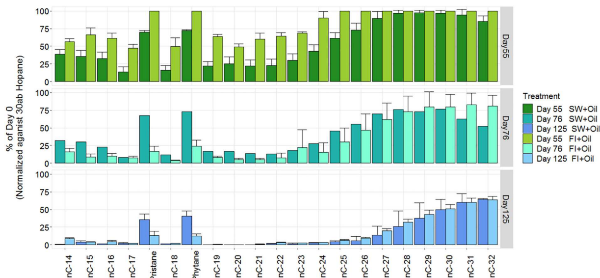
Fig. 1. Degradation of target n-alkanes in dispersed oil with frazil ice (FI + oil), and dispersed oil w/o frazil ice (SW + oil). The losses are shown as percentages of day 0, after normalization against 30ab Hopane. Different colours represent the sampling days from day 0 to day 125.
