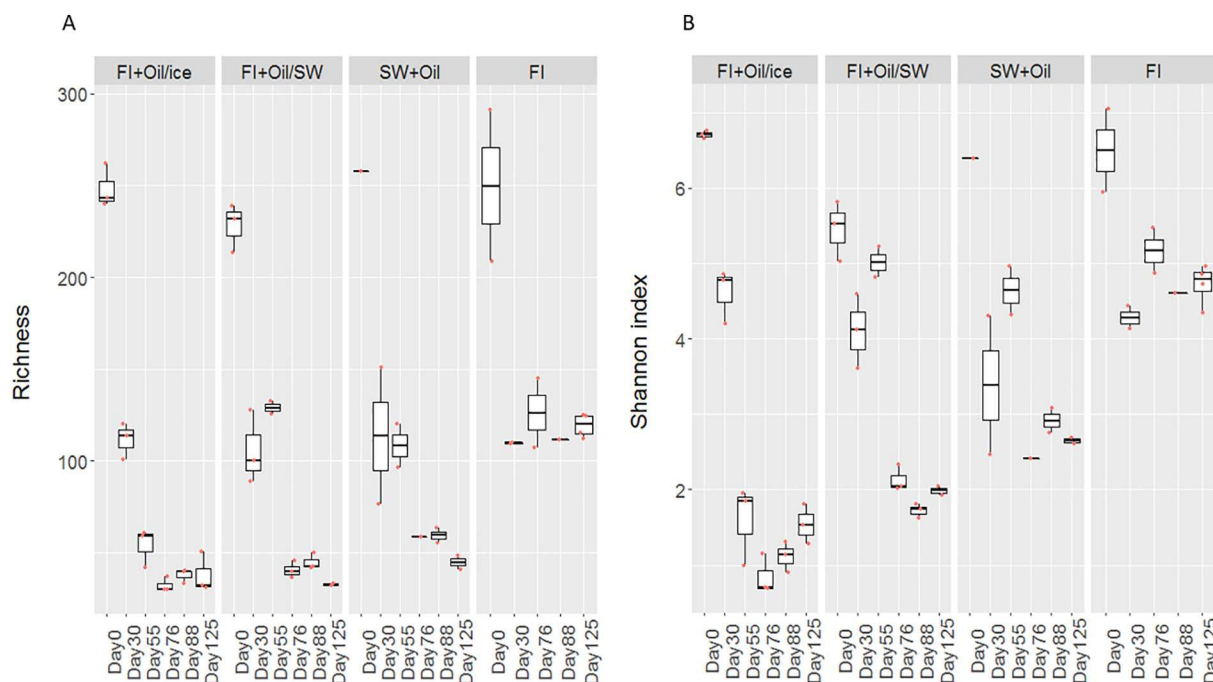
Fig. 4. Changes in species richness (A) and in the Shannon index diversity (B) during the 125 days of incubation, in the different treatments; dispersed oil with frazil ice (FI+oil/SW and FI+oil/ice); dispersed oil w/o frazil ice (SW+oil); and seawater without oil with frazil ice (FI).
