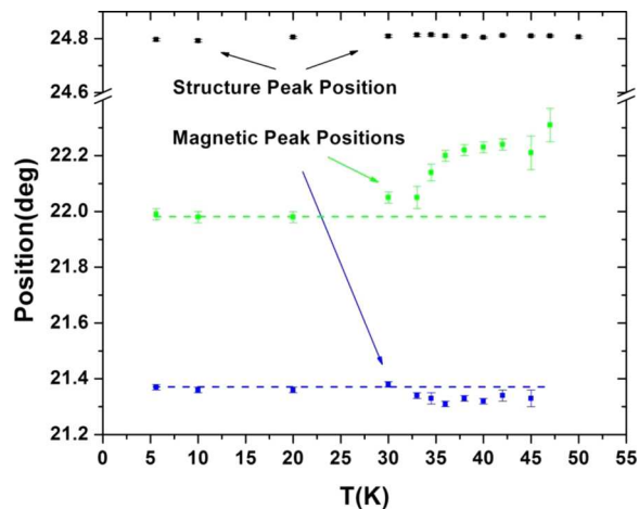
Figure 7. Temperature dependence of selected structural and magnetic peaks positional shifts.
