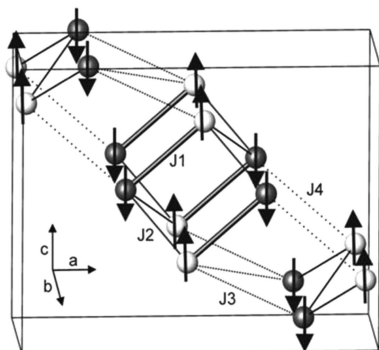
Figure 12. Most likely magnetic structure for BaYFeO 4 from the spin dimer results.
