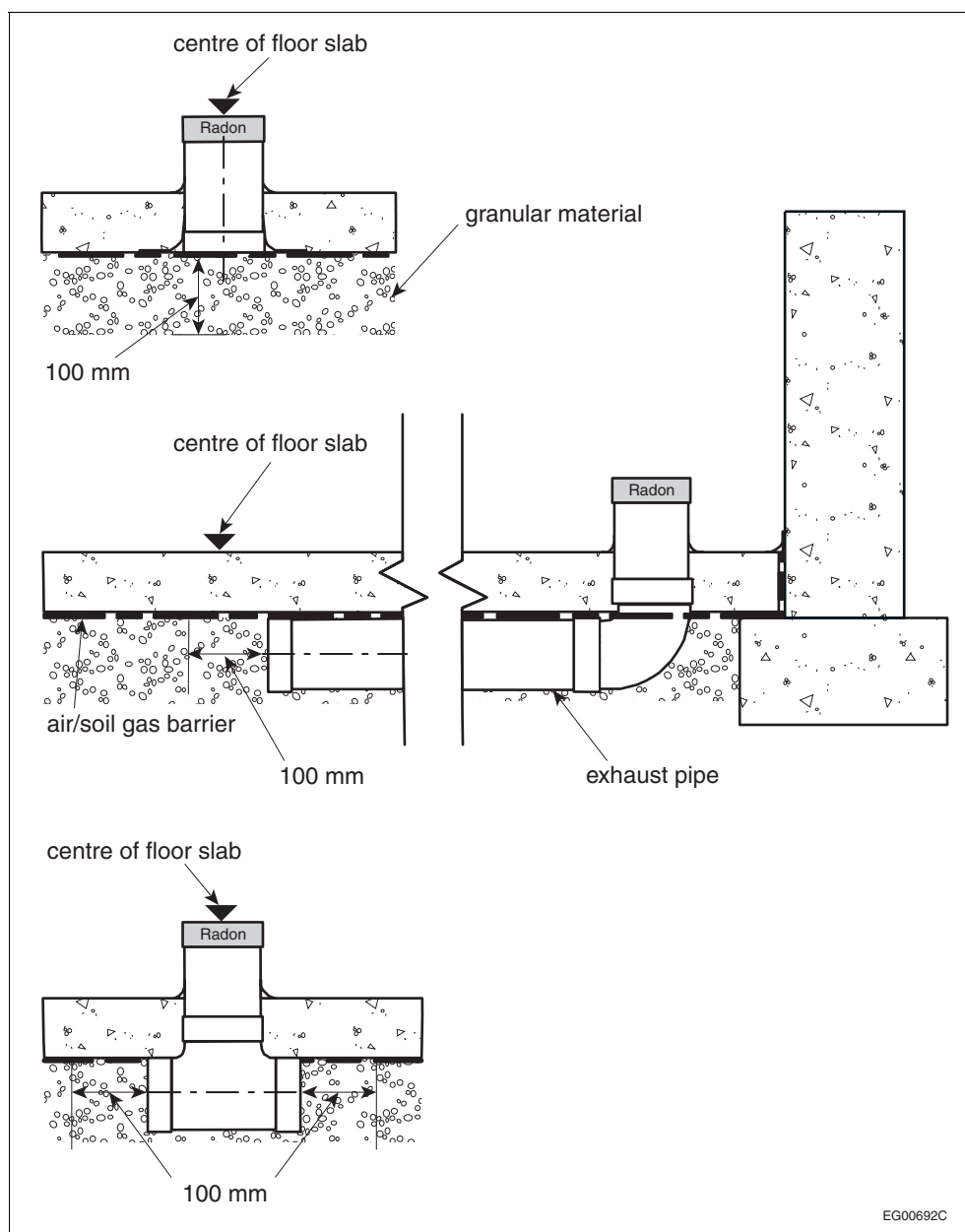
Figure A-9.13.4.3.(2)(b) and (3)(b)(i)
