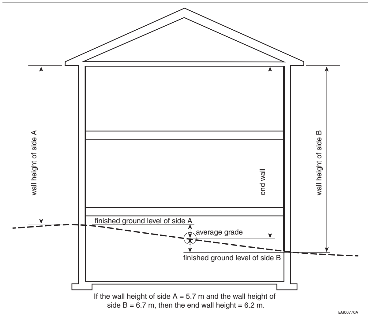
Figure A-9.36.2.3.(2) and (3)
