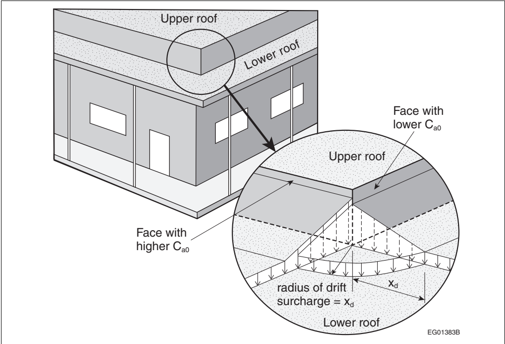
Figure 4.1.6.8.-B Snow load at inside corner Forming Part of Sentence 4.1.6.8.(2)
