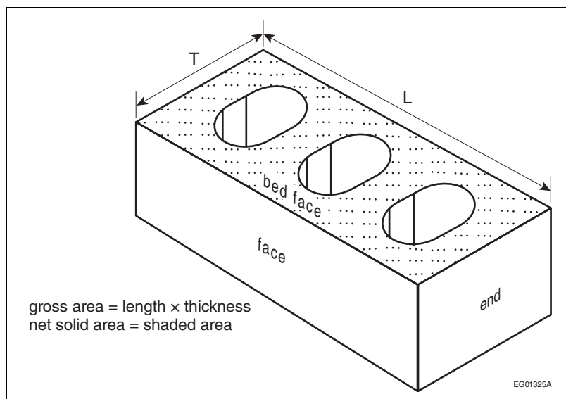
Figure A-1.4.1.2.(1)-B Net solid area of masonry unit
