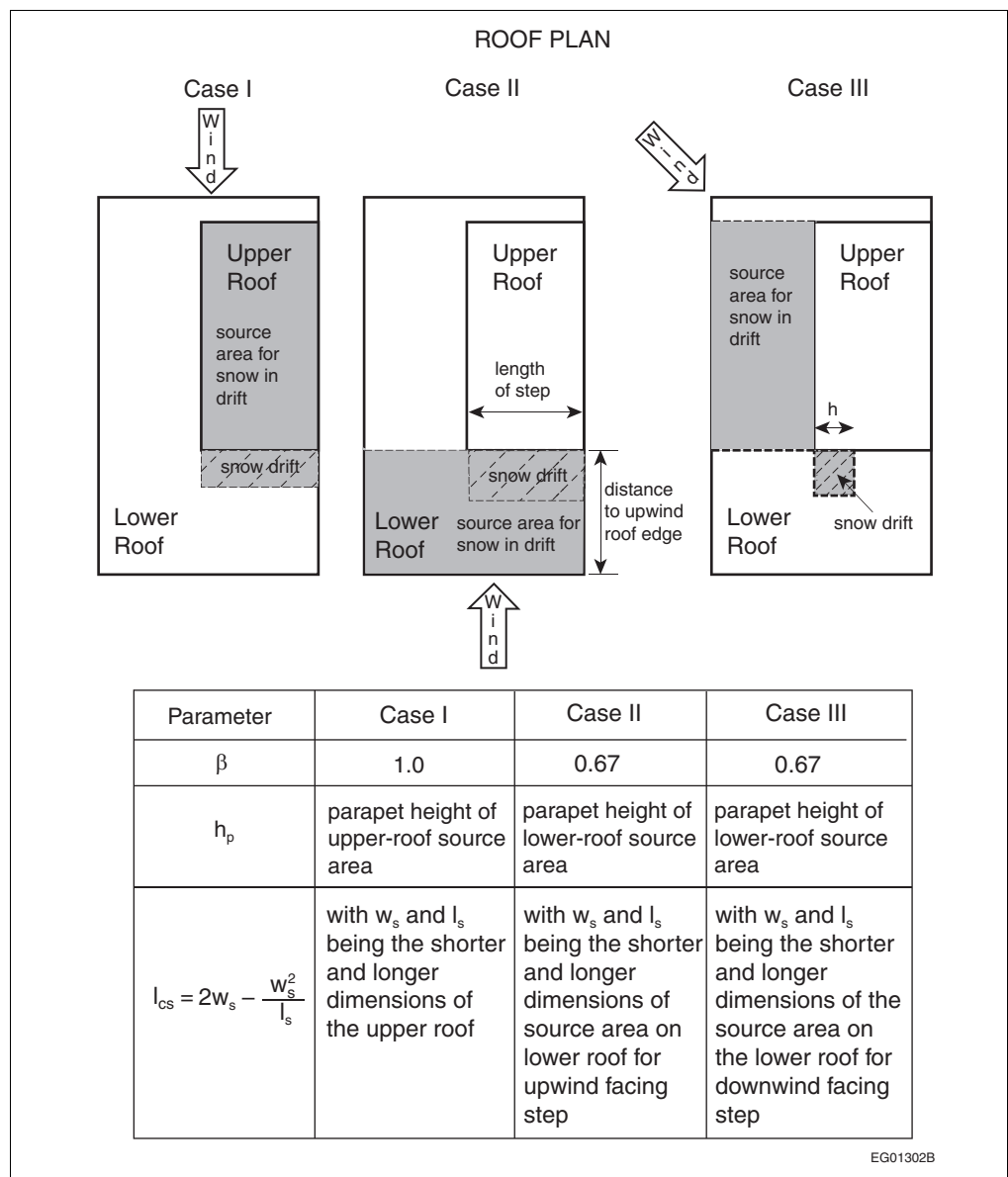
Figure 4.1.6.5.-B Snow load cases I, II and III for lower level roofs Forming Part of Sentences 4.1.6.5.(1), (3) and (4)
