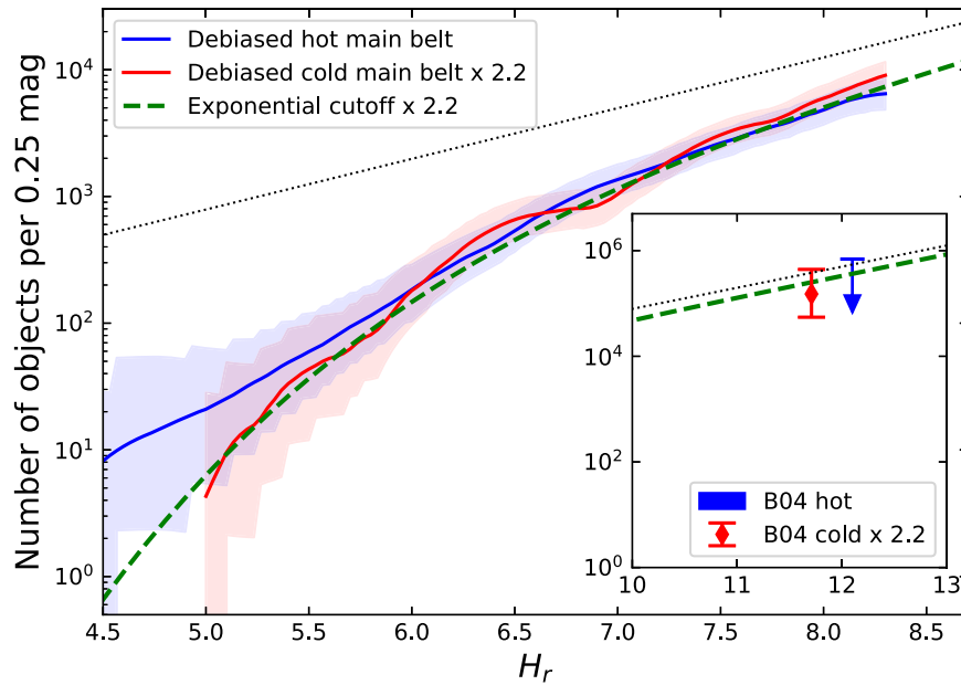
Figure 2. Similar to Figure 1, whereas here the debiased cold component estimates and uncertainties have been scaled upward by a factor of 2.2. The green dashed line shows the Kavelaars et al. (2021) cold-population exponential cutoff fit (with large- H asymptotic slope of 0.4), also scaled upward by a factor of 2.2. The inset shows the continuation of the scaled exponential cutoff fit at larger/fainter H_r ; the red error bar gives the 95% confidence range from the detection of three cold TNOs using HST by Bernstein et al. (2004) and is compatible with the above extrapolation. The inset’s blue arrow shows the 95% confidence upper limit from the nondetection of hot population TNOs in that same HST study. For H_r > 5.5 the shape of the hot and cold populations’ curves are surprisingly similar, which hints at similar formation processes. The black dotted line is a reference exponential with logarithmic slope \alpha = 0.4 to help see how the exponential taper deviates from a single exponential.
