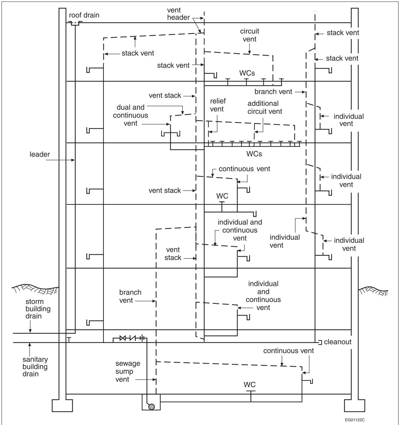
Figure A-1.4.1.2.(1)-G Venting System
