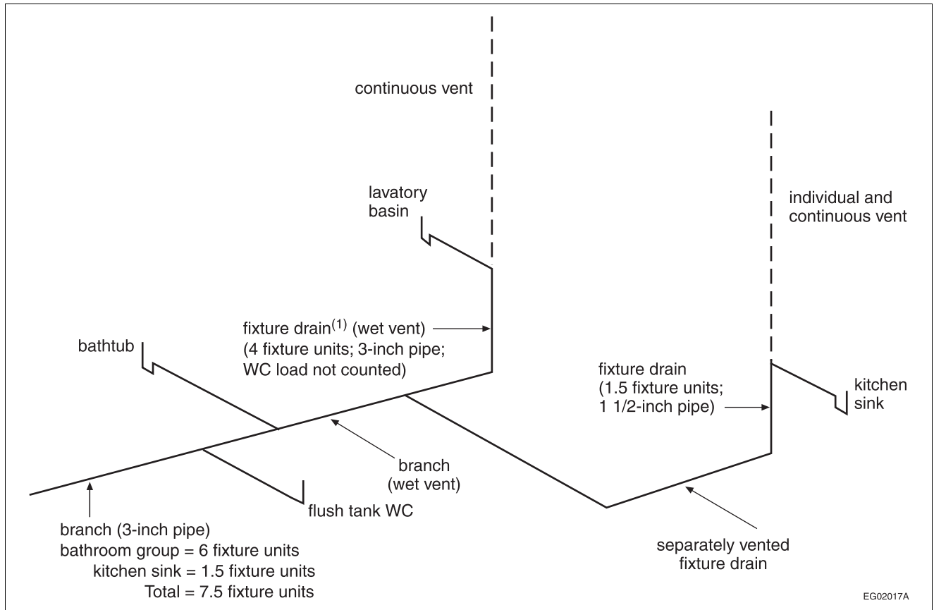
Figure A-2.5.2.1-E Example of Wet Venting Described in Clause 2.5.2.1.(1)(f)
