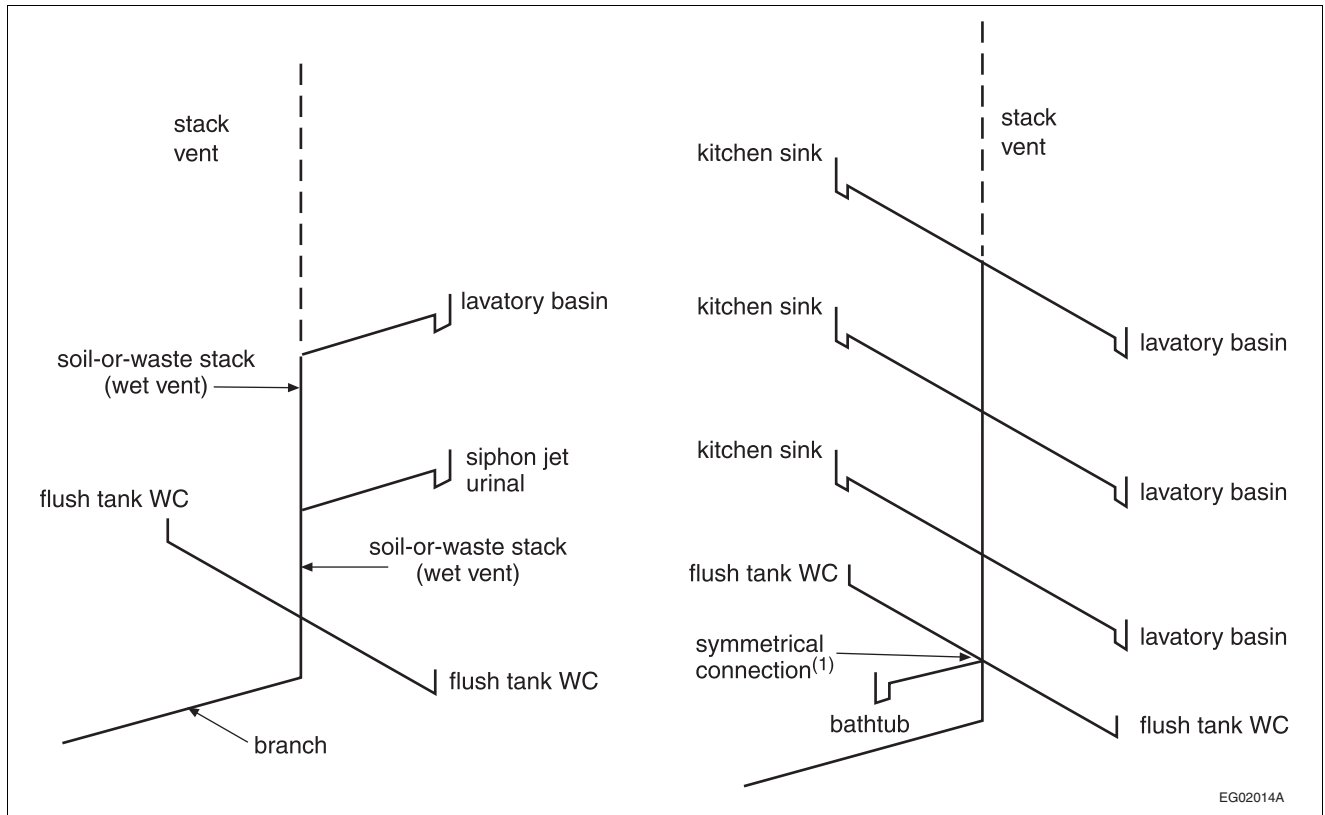
Figure A-2.5.2.1.-B Example of Wet Venting Described in Clause 2.5.2.1.(1)(c)
