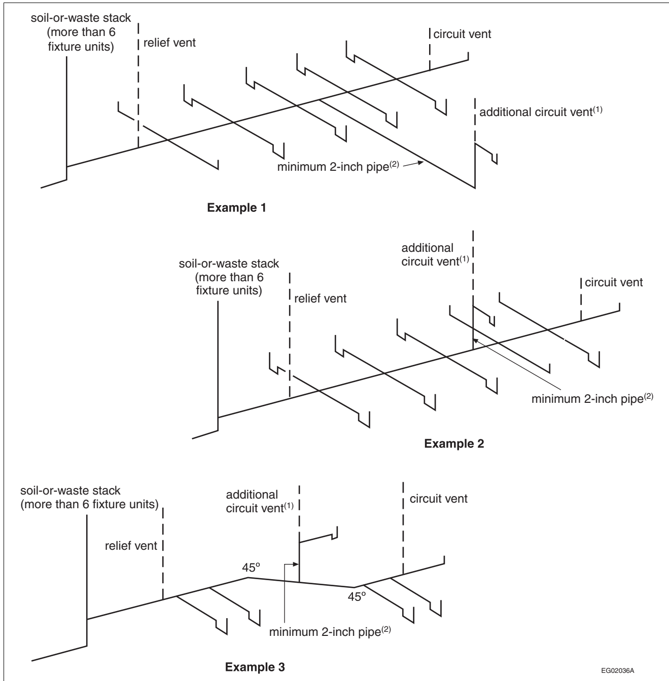
Figure A-2.5.3.1.-I Example of Circuit Venting Described in Sentence 2.5.3.1.(7)
