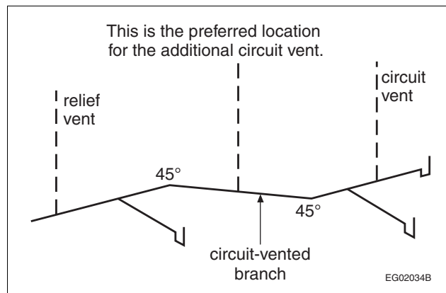
Figure A-2.5.3.1.-G Example of Circuit Venting Described in Clause 2.5.3.1.(6)(a)
