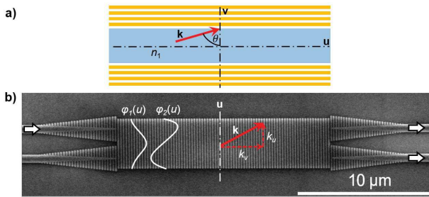
Fig. 2. (a) When light is incident from a homogenous waveguide core onto a birefringent cladding material, such as an SWG, the conditions for total internal reflection are relaxed, and a stronger light confinement is possible. (b) Scanning electron microscope image of a multimode interference (MMI) beam-splitter with measured bandwidth of more than 300 nm in the telecom 1.55 \mu\text{m} band. The SWG in the central region is anisotropy-engineered to optimize propagation constants of the Bloch-Floquet modes for broadband operation. The four input/output tapered regions provide a smooth transition to the interconnection single mode waveguides.
