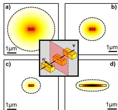
Fig. 3. Electric field of the fundamental TE Bloch-Floquet mode propagating along the v axis in an SWG waveguide. The fields are shown in the central plane of the Si segment (see the inset). Silicon thickness and grating period are t_{\text{Si}} = 220 nm and \Lambda = 200 nm. Waveguide width and duty cycle are: (a) w = 400 nm, f = 30\% , (b) w = 400 nm, f = 50\% , (c) w = 400 nm, f = 70\% , (d) w = 3 \mu\text{m} , f = 50\% . Outside the dotted curves the field amplitudes are below 2% of the maximum value.
