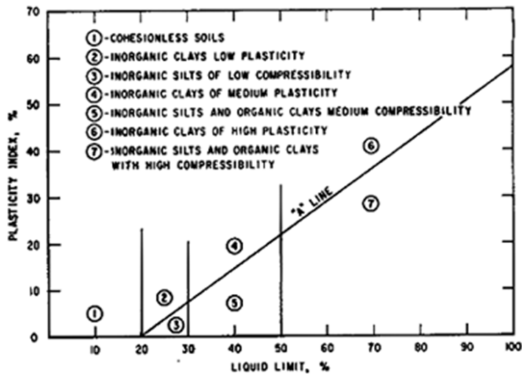
Figure 1. Plasticity chart (after A. Casagrande)
