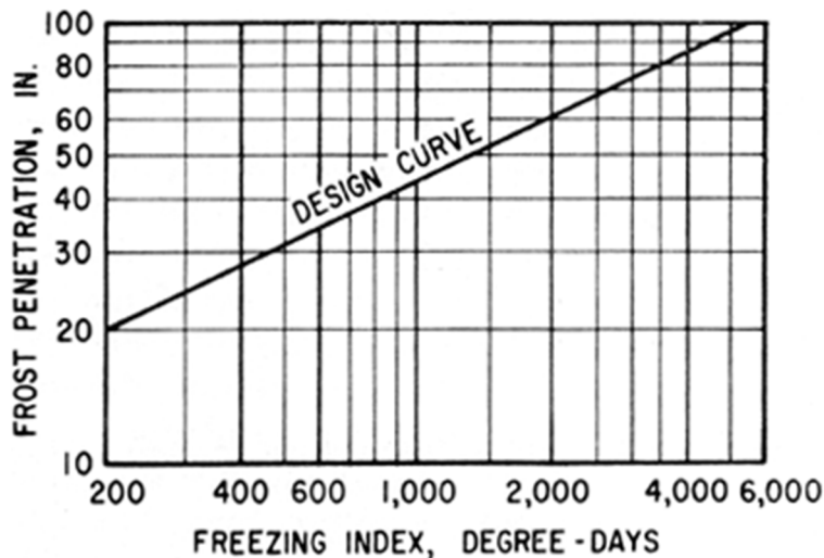
Figure 1. "Design Curve" of observed frost penetration in excavations.
