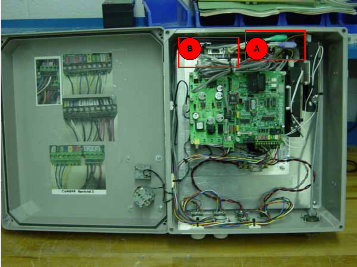
Figure 7. Computer Enclosure (Inside).
