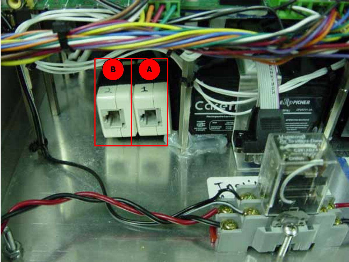
Figure 8. Ethernet/data connection between the cameras and the computer inside the computer enclosure.
