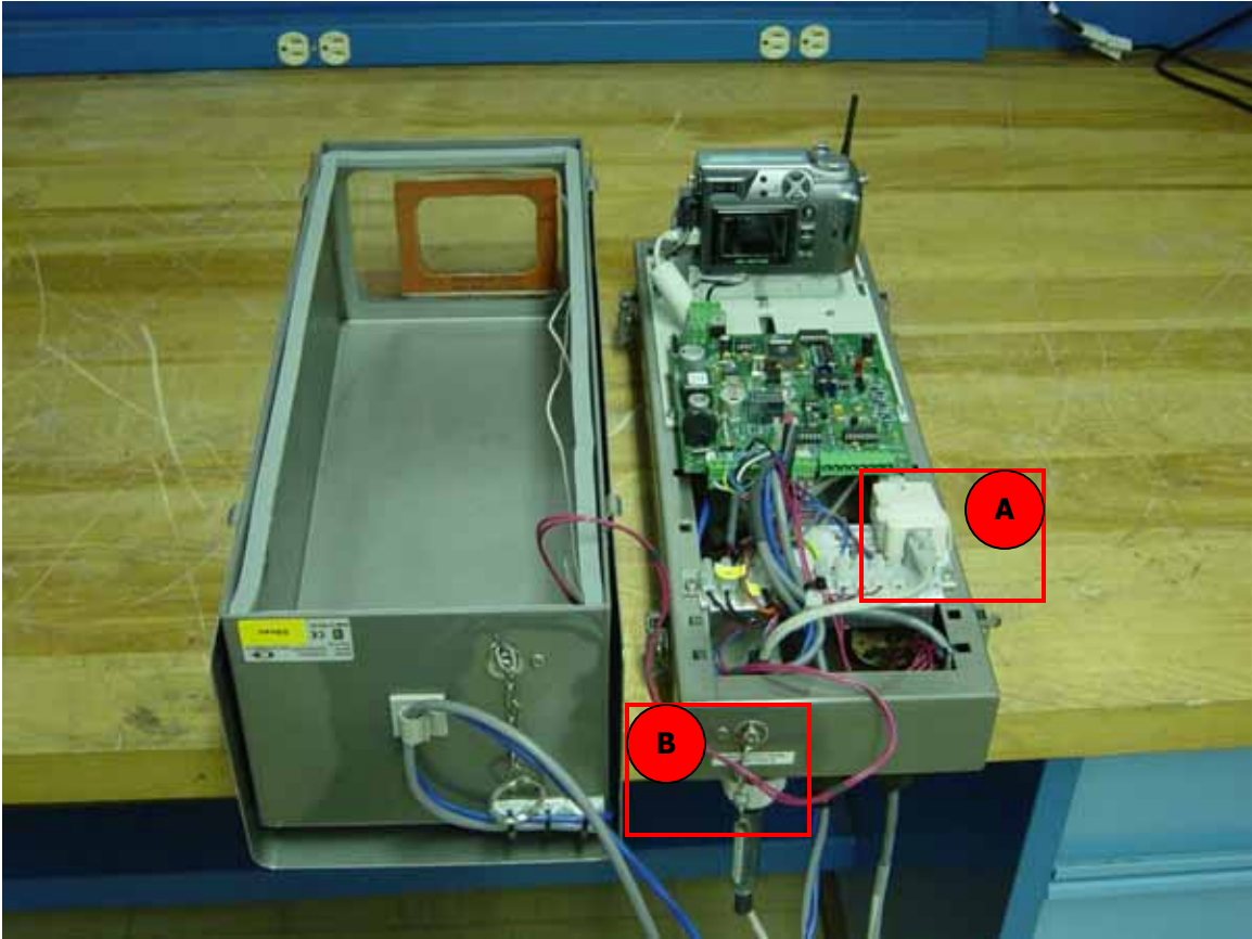
Figure 11. Camera Enclosure (Inside).
