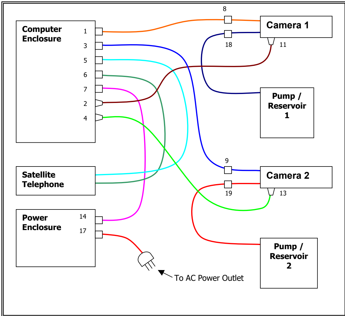
Figure 1. Connection Diagram.
