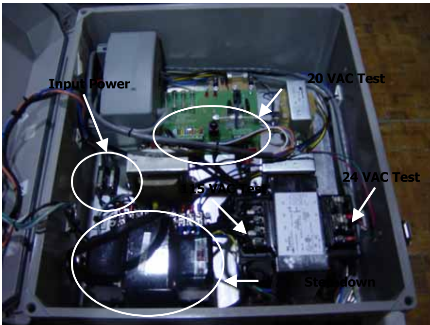
Figure 17: Power Enclosure After Modifications
