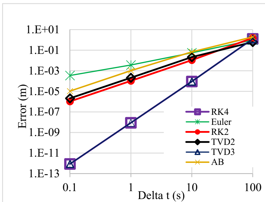
Fig. 6. Local error of the numerical solution of Test 1 (Table 3) at t = 10 s for the tested numerical schemes in this study in the log-log coordinate.
