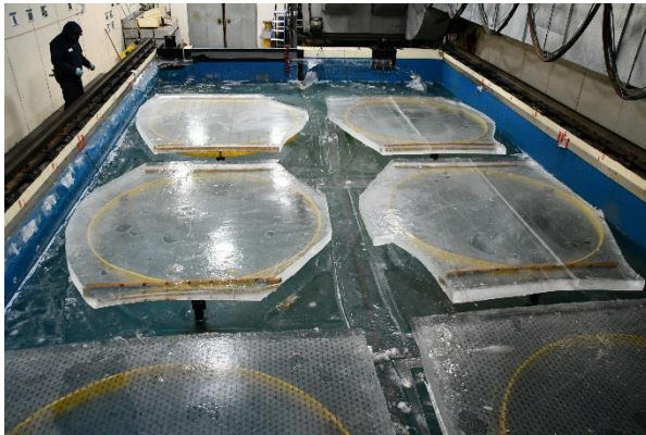
Figure 47: Individual plates after having been cut and the water level having been lowered, bringing them down and allowing them to rest directly on the test frames. Person for scale upper left corner.
