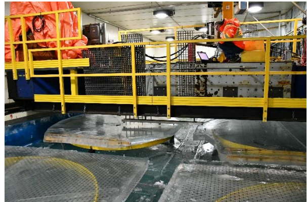
Figure 48: The carriage has been move to the location of a test. Below it is the instrumentation used to monitor the ice loading event and the ice response. Person with orange jacket for scale, upper right.
