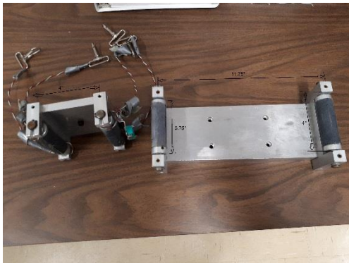
Figure 16: The load application frame (see Figure 18 for scale).
