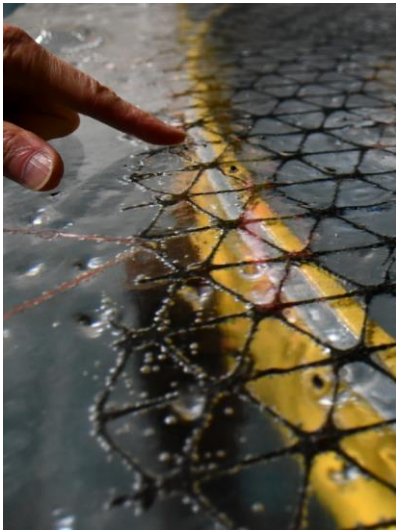
Figure 61: Polypropylene geogrid inside the ice before test E1 – note the presence of air bubbles along the ice-material interface.
