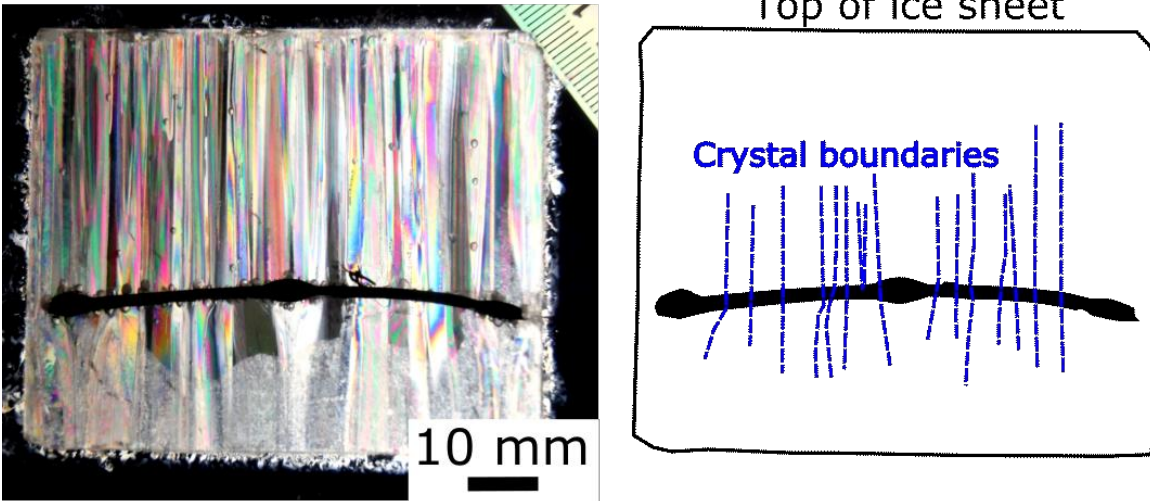
Figure 35 - Left) Thin section in cross-polarized light across the thickness of an ice cover, with the enclosed Tensar geogrid. Right) Outline of crystal boundaries and membrane. Note how the crystal are able to grow through the membrane, i.e. the membrane does not promote a discontinuity.
