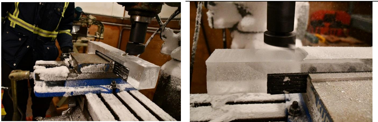
Figure 10 (left and right): Shaping the ice beams into the target testing dimensions with a lathe.
