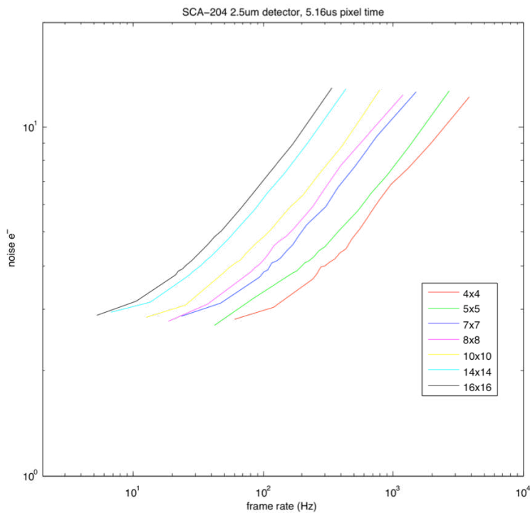
Fig. 5. Preliminary results - HxRG detector read noise vs. frame rate for window sizes
