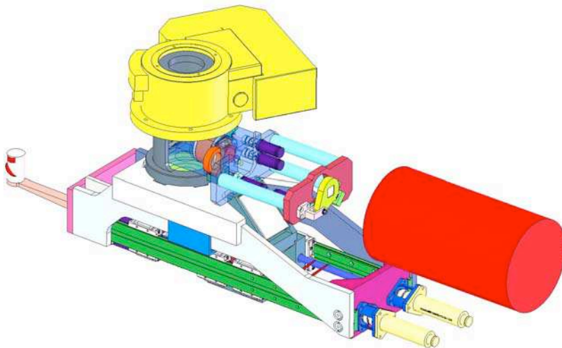
Fig. 4. Theta-R probe mechanics design
