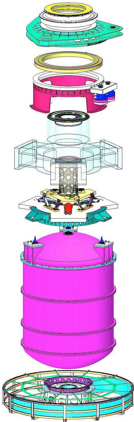
Fig. 6. Exploded view of macro mechanics
