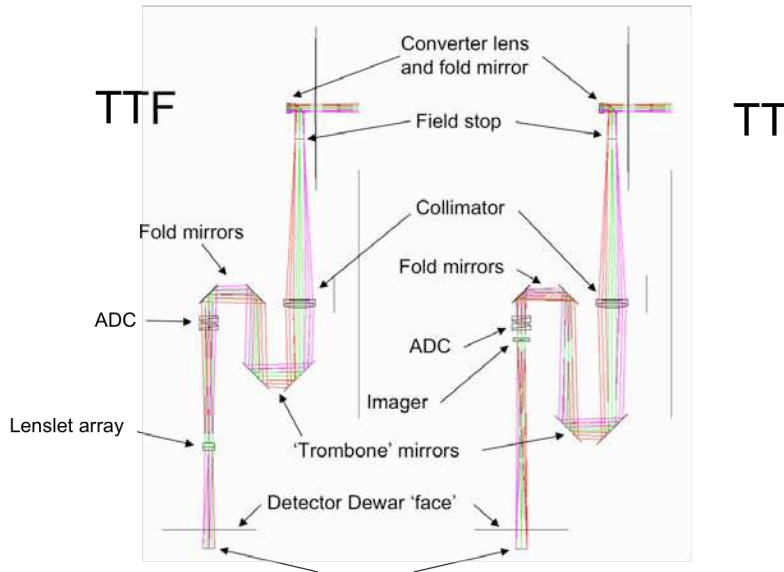
Fig. 3. Theta-R probe optics design with TT and TTF function change
