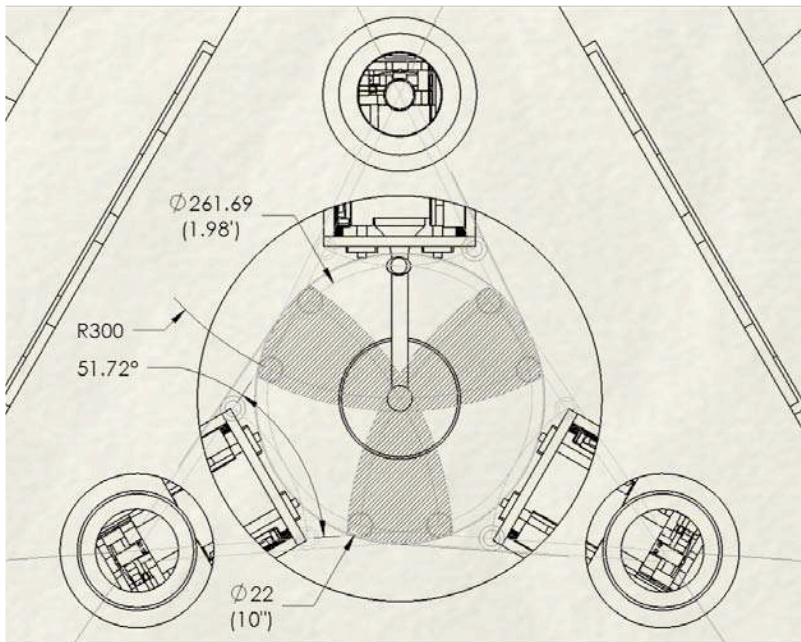
Fig. 2. Plan view of theta-R probe geometry
