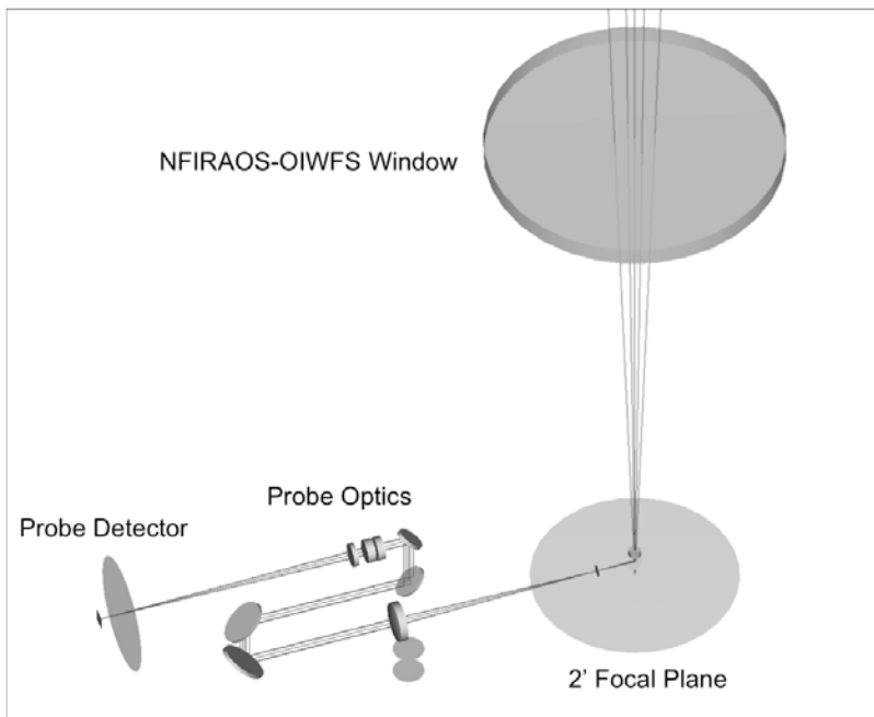
Fig. 1. General optical arrangement with respect to NFIRAOS delivered focal plane
