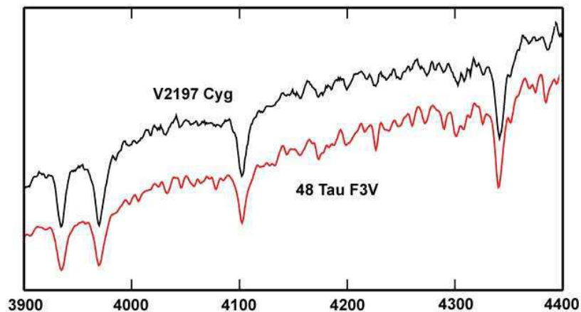
Figure 2. Classification spectra.
