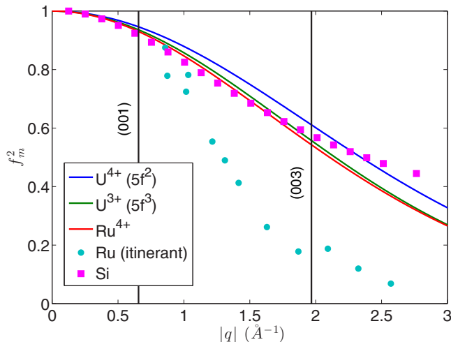
FIG. 4. (Color online) Square of the magnetic form factors for several types of spin densities as a function of scattering wave vector |\mathbf{q}| . The first three curves correspond to localized ionic states of uranium [ U^{4+} ( 5f^2 ) and U^{3+} ( 5f^3 )] and ruthenium ( Ru^{4+} ), and are described by Eq. (B1). We also roughly approximate the possible spin density that could be associated with Ru- or Si-derived conduction bands, for example as might be appropriate for conduction electrons in the hastatic order theory [11]. The data for Si are those of the x-ray atomic scattering factor squared, which measures the Fourier transform of the total electron density (Ref. [35]).
