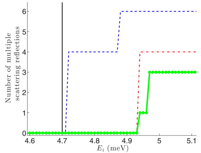
FIG. 7. (Color online) The number of reflections accessible by multiple scattering when the scattering geometry is set to measure (001) (blue dashed line), (003) (red dot-dashed line), and (101) (green line with symbols) for different incident energies ( E_i ), with \mathbf{k}_i and \mathbf{k}_f spanning the ( HOL ) scattering plane. At E_i = 4.7 meV (black solid line), no multiple scattering is possible for these configurations within a resolution tolerance of 0.05 \text{ \AA}^{-1} .
