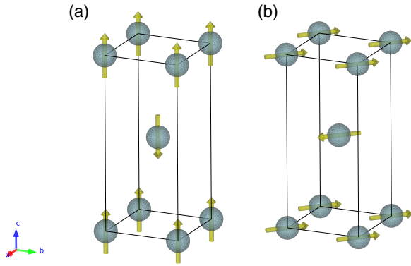
FIG. 1. (Color online) Schematic of magnetic ordering for the (a) known out-of-plane magnetic moments ( \mu_{\parallel} ) in the SMAF phase below T_{\text{HO}} , and (b) proposed in-plane magnetic moments ( \mu_{\perp} ) from Refs. [9–11].
