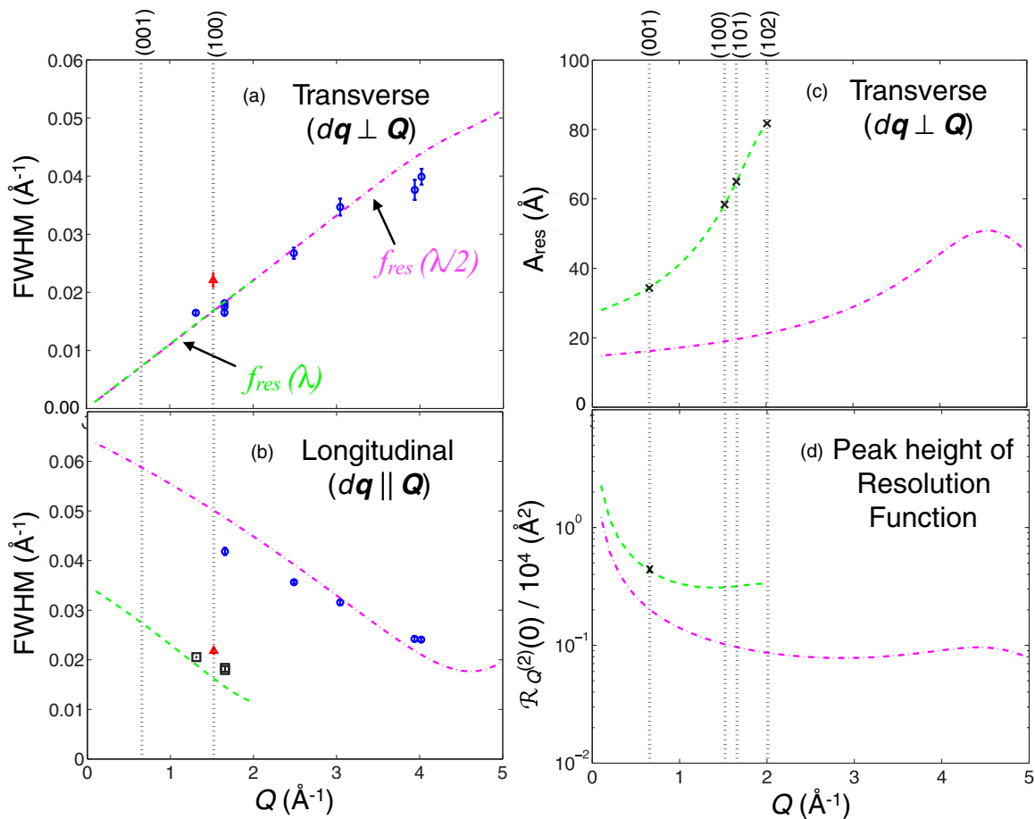
FIG. 5. (Color online) (a) and (b) Calculated and measured FWHM of Bragg peaks as a function of scattering wave number q , for transverse and longitudinal scans. The blue circles ( \lambda/2 ) and black squares ( \lambda ) show the measured FWHM for nuclear peaks, and the red triangle shows the measured FWHM for the (100) magnetic peak (error bars represent half of the 95% confidence interval resulting from fits to a Gaussian line shape). The calculated FWHM ( f_{\text{res}} ) are based on resolution function calculations for the following instrumental configuration: incident beam divergence of 60'/k_i , PG(002) vertically focused monochromator, 80' collimators before and after the sample, PG(002) flat analyzer, and 33' sample mosaic. For Q < 2 \text{ \AA}^{-1} the FWHM are measured and calculated (green dashed line) for incident neutrons with k_i = 2\pi/\lambda_{PG(002)} = 1.8733 \text{ \AA}^{-1} . For Q > 2 \text{ \AA}^{-1} , the FWHM are shown (pink dot-dashed line) for k_i = 2\pi/(\lambda_{PG(002)}/2) = 3.7465 \text{ \AA}^{-1} . (c) Calculated areas of the resolution function ( A_{\text{res}} ) for transverse scans as a function of Q , for the instrumental configuration above (green dashed line is for \lambda_{PG(002)} , pink dot-dashed line is for \lambda_{PG(002)}/2 ). (d) Peak height of the normalized two-dimensional resolution function [Eq. (A10)]. The black crosses show the values used for determining the measured cross sections at the specified zone centers.
