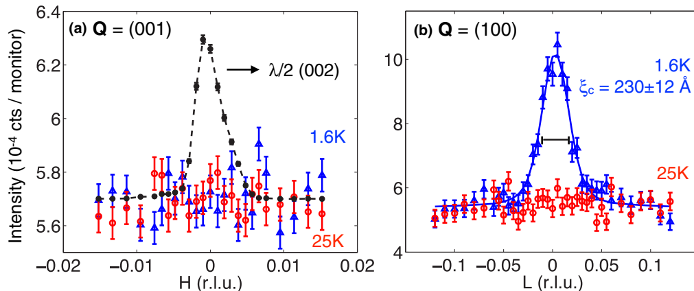
FIG. 3. (Color online) Transverse \mathbf{q} scans at two positions, (a) (001) and (b) (100), which would correspond to in-plane and out-of-plane magnetic ordering, respectively. Only the (100) position shows a magnetic Bragg peak upon cooling through T_{\text{HO}} = 17.5 K. A transverse scan performed at the same position as (001) but without the higher-order filters in the beam [i.e., intentionally including \lambda/2 contamination from the (002) nuclear Bragg peak] indicates the correct position of the scan in reciprocal space [black dashed line in (a)], scaled down by a factor of 7200. The horizontal bar in (b) represents the calculated full width at half maximum of the instrumental resolution (see Fig. 5). The monitor count rate was 6100 counts/s. Error bars represent one standard deviation.
