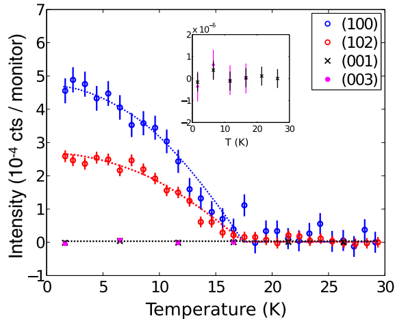
FIG. 2. (Color online) Temperature dependence of the peak intensity at several candidate magnetic Bragg peaks. The inset shows the temperature dependence of the peaks which would correspond to in-plane magnetic ordering, on a finer intensity scale. Dotted lines are guides to the eye. The monitor count rate was 6100 counts/s. Error bars represent one standard deviation.
