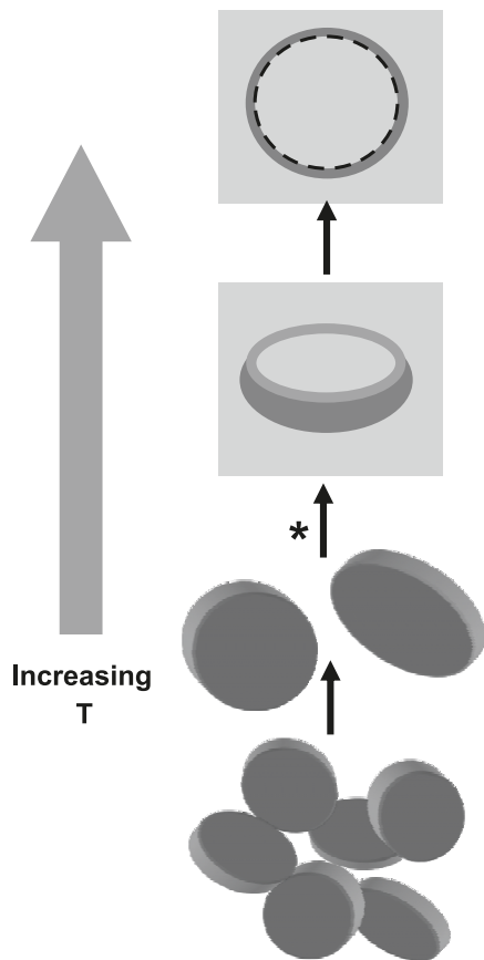
Fig. 2. Schematic describing the various morphologies as a function of temperature for a DMPC–DHPC–DMPG lipid mixture. The asterisk indicates the stage at which ULV size is determined. T^* is a function of total lipid concentration.
