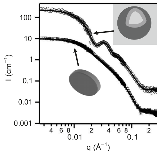
Fig. 1. Typical SANS data of low-polydispersity ULVs (circles) at 45 °C and bicelles (triangles) at 10 °C. The data were best fit using a spherical-shell model [15] and a core-shell discoidal model [16] (solid lines).
