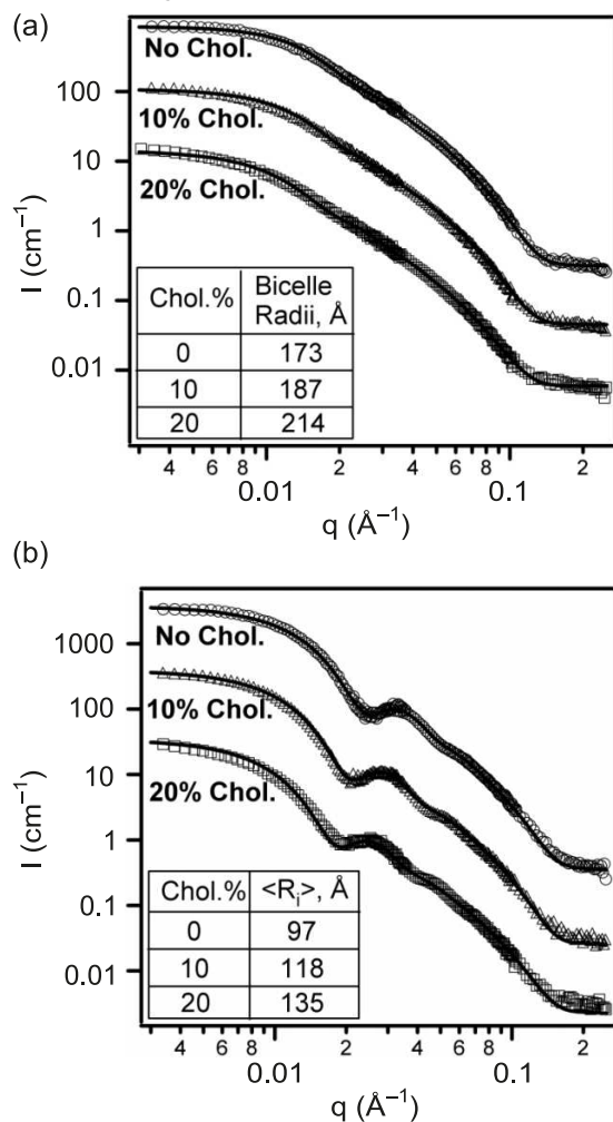
Fig. 4. (a) 10 °C and (b) 50 °C SANS data of DMPC–DHPC–DMPG doped with various molar ratios of cholesterol i.e., [Chol]/[DMPC]: 0 (circles), 10% (triangles), 20% (squares). At 10 °C, bicelles are present, which transform into ULVs at 50 °C. Solid curves are the best fits to the data. Best-fit parameters are tabulated in the inset to the figure.
