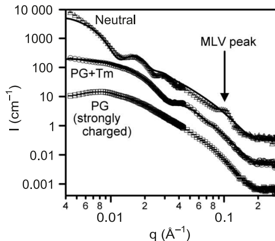
Fig. 3. SANS data of a neutral Q = 3.2 and R = 0 (DMPC–DHPC) (triangles) lipid mixture, a Q = 3.2 and R = 0.067 (DMPC–DHPC–DMPG) weakly charged lipid mixture doped with \text{TmCl}_3 ( [\text{TmCl}_3]/[\text{DMPC}] = 0.033 ) (circles), and a strongly charged Q = 3.2 and R = 0.067 (DMPC–DHPC–DMPG) lipid mixture (squares). In all cases, lipid concentration is 0.25 wt% and temperature is 45 °C. For R = 0 and 0.067 mixtures, the data were fit using the spherical-shell model. An MLV peak at q \sim 0.1 \text{ \AA}^{-1} for the neutral mixture was also observed and could not be fit by the model. The strongly charged sample showed the characteristic “bicelle” scattering pattern, the result of strong interparticle interactions. The data and fits to the data are rescaled for clarity of viewing.
