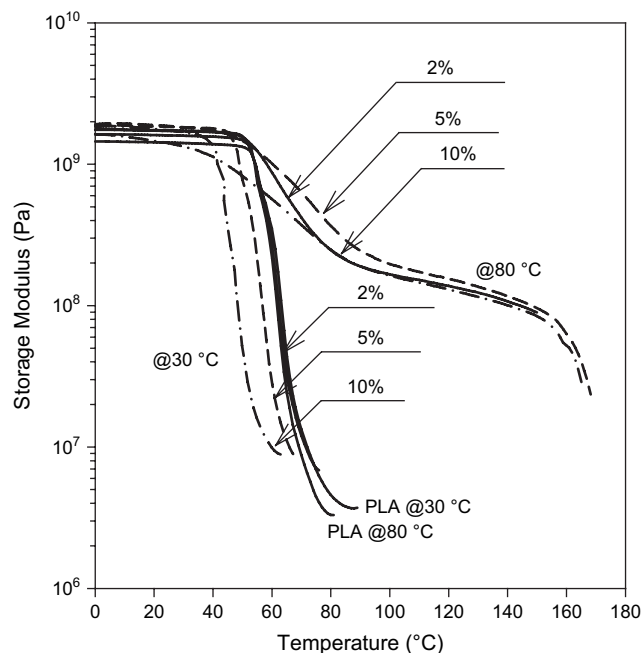
Fig. 9. Effect of temperature on the storage modulus for PLA control and for formulations comprising 1% talc with 2, 5 and 10% PEG, molded at 30 and 80 ^{\circ}\text{C} .
