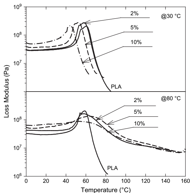
Fig. 10. Effect of temperature on the loss modulus for PLA control and for formulations comprising 1% talc with 2, 5 and 10% PEG, molded at 30 and 80 ^{\circ}\text{C} .
