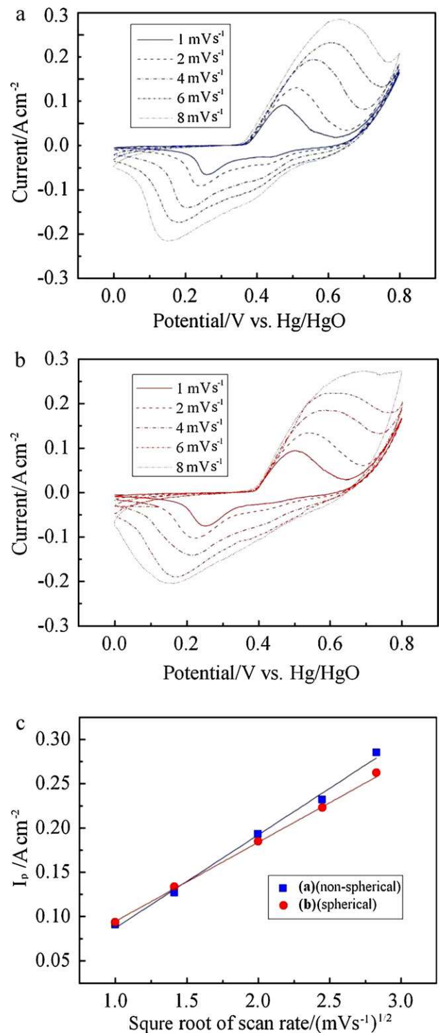
Fig. 6. Cyclic voltammograms of (a) non-spherical \text{Ni}(\text{OH})_2 and (b) spherical \text{Ni}(\text{OH})_2 at various scan rates. (c) Linear relationship between the cathodic peak current ( I_p ) and square root of scan rate for (a) non-spherical \text{Ni}(\text{OH})_2 and (b) spherical \text{Ni}(\text{OH})_2 .
