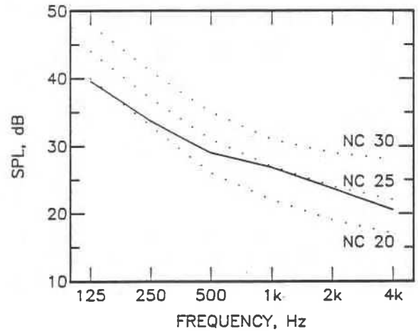
Figure 6. Mean Octave Band Residual Background Noise Levels versus Frequency —, and NC contours - - -.
