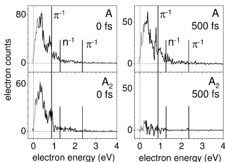
Figure 4. FEICO spectra of the adenine monomer and the adenine dimer, recorded at zero and 500 fs delay time between the 266 nm pump and 800 nm probe pulses. The long vertical lines indicate the electron energy corresponding to the adenine vertical ionization potential into D_0 ( \pi^- ) by a three photon probe process. The short vertical lines indicate the corresponding electron energies associated with ionization into the D_0 ( \pi^- ) and D_1 ( n^- ) states by a four photon probe process.
