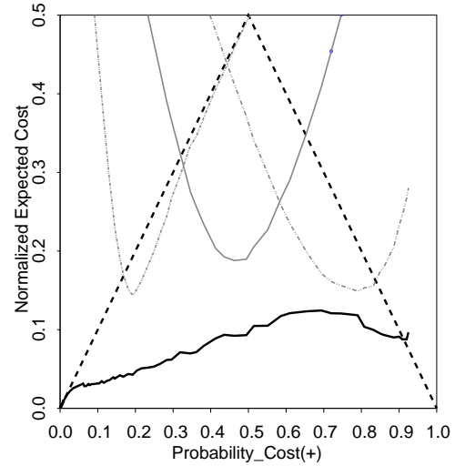
Figure 6: Using a Predictive Algorithm
