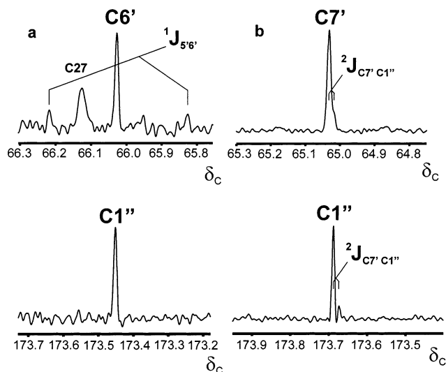
FIGURE 3. Portions of the Lorentz–Gauss resolution-enhanced 125.7 MHz ^{13}\text{C} NMR spectra of 5 and 6 enriched from [1,2-^{13}\text{C}_2] acetate, showing resonances for (a) C6' and C1'' of 5 and (b) for C7' and C1'' of 6 . The latter peaks show isotopically shifted ^{13}\text{C} – ^{13}\text{C} doublets ( ^2J_{\text{COC}} \approx 2.5 Hz) indicating that O has been inserted in 6 between two carbons of a previously intact unit derived from acetate. The relative intensity of these doublets is the same as for ^1J_{\text{CC}} doublets for carbons derived from intact acetate units.
