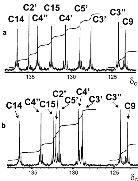
FIGURE 2. Portions of the 125.7 MHz ^{13}\text{C} NMR spectra of (a) 5 and (b) 6 enriched from [1,2-^{13}\text{C}_2] acetate and satellites due to incorporation of intact ^{13}\text{C} – ^{13}\text{C} units, at C14, C4'', C15, C4', C5', and C3'. Integrals show uniform ^{13}\text{C} enrichment at these carbons and a lower enrichment at C2', corresponding to incorporation of scrambled label only. In 4 , C2' was shown previously 13,15 to originate from glycolate. Spectrum a was recorded under “quantitative” conditions with suppressed NOE, whereas spectrum b was obtained without NOE suppression. The latter spectrum yielded relative enrichments of proton-bearing carbons close to those from a “quantitative” spectrum of the same compound, indicating that the former in particular was yielding reliable enrichment values.
