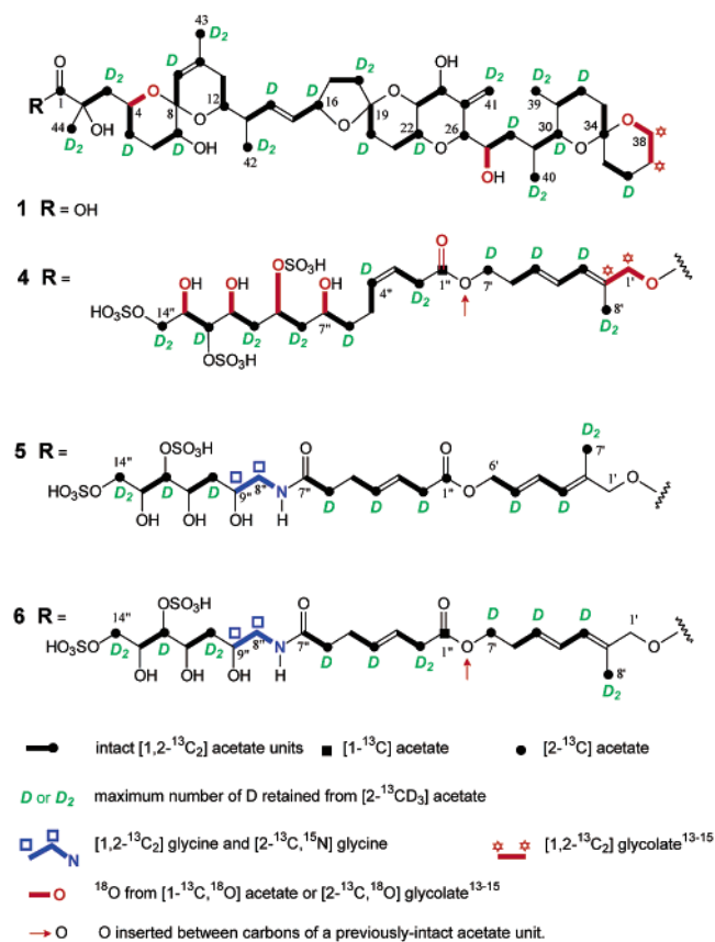
FIGURE 1. Structures of okadaic acid ( 1 ), DTX-4 ( 4 ), DTX-5a ( 5 ) and DTX-5b ( 6 ) showing incorporation of stable isotope labels determined from previous experiments (for 1 and 4 ) 13–15 and from the experiments in this report (for 5 and 6 ).
