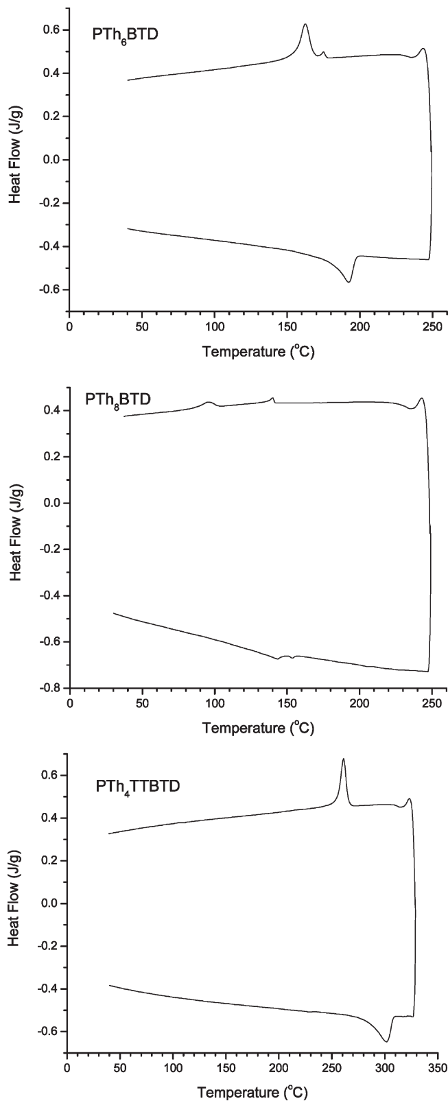
Figure 3. Second scan DSC curves of PTh 6 BTD and PTh 8 BTD. PTh 4 TTBTD at a heating/cooling rate of 10 °C under nitrogen.
