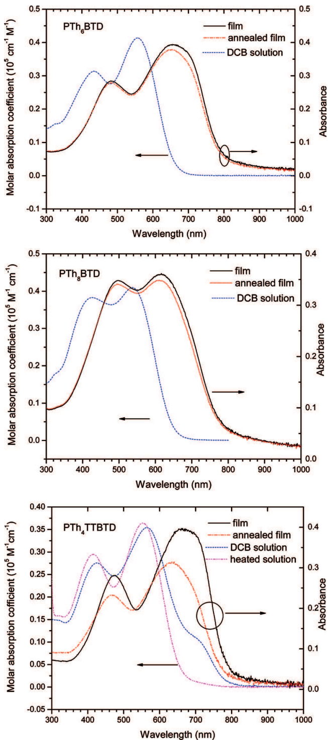
Figure 2. Absorption spectra of polymers PTh 6 BTD, PTh 8 BTD, and PTh 4 TTBTD in 1,2-dichlorobenzene solution and in solid film state (50 nm thick). The annealing temperatures for PTh 6 BTD, PTh 8 BTD, and PTh 4 TTBTD films are 120, 100, and 200 °C, respectively.
