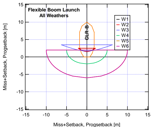
Figure 8. Flexible boom: Splashdown area boundaries.
