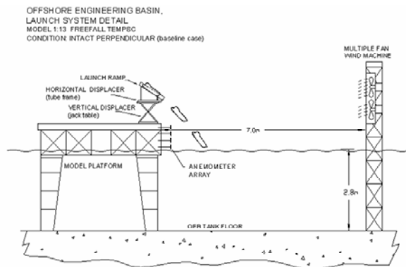
Figure 2. Test setup: Free-fall lifeboat system.
