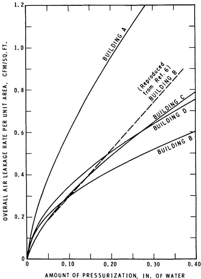
Fig. 9 Overall air leakage rate per unit area vs building pressurization
