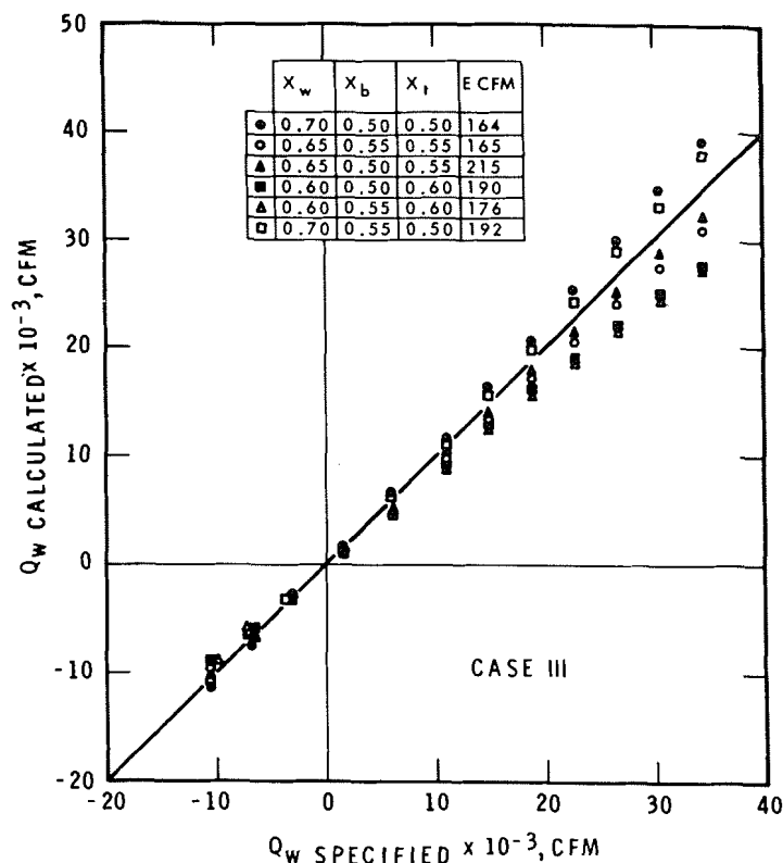
Fig. 3c Calculated exterior wall air leakage rate vs specified exterior wall air leakage rate for various standard errors of estimate
