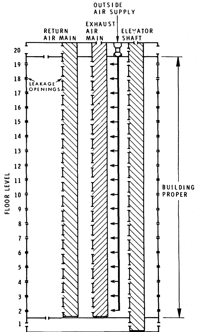
Fig. 2 Computer-simulated building
