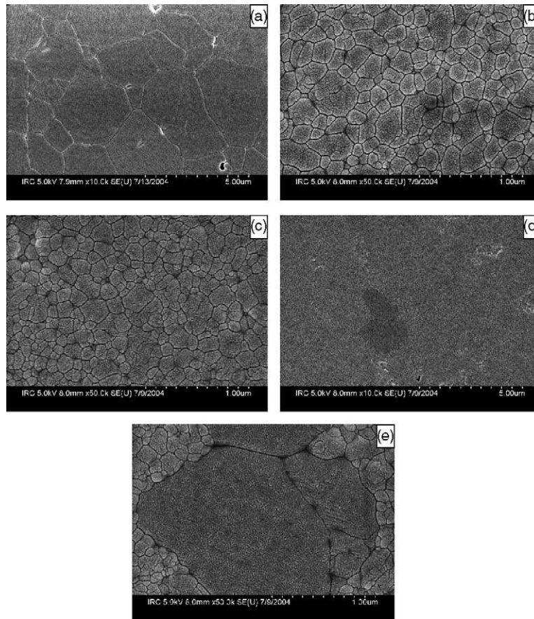
Fig. 6. SEM microstructures of (\text{CeO}_2)_{1-x}(\text{STO})_x after thermal etching at 1200\text{ }^\circ\text{C} for 24 min: (a) x = 0 , (b) x = 0.1 , (c) x = 0.2 , (d and e) x = 0.2 , the dark STO and light \text{CeO}_2 phases were confirmed by EDX.
