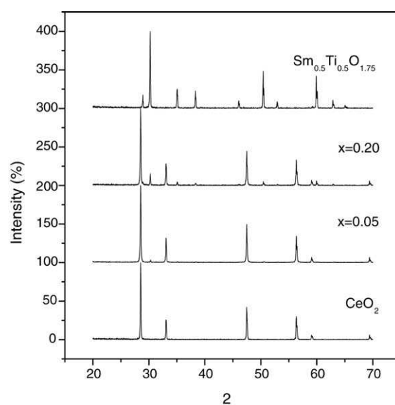
Fig. 1. X-ray diffraction patterns for (CeO 2 ) 1-x (STO) x ceramics sintered at 1300 °C.
