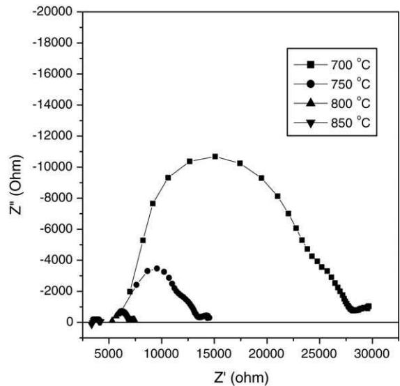
Fig. 5. The ac complex impedance plots for (\text{CeO}_2)_{0.95}(\text{STO})_{0.05} ceramics as a function of temperature.
