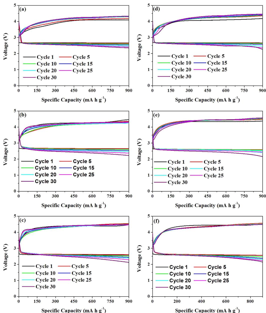
Figure 4. Cycling performance of f-NiS (a–c) and r-NiS (d–f) based electrodes with controlled capacity of 900 mA h g −1 at various current densities (75 (a,d), 150 (b,e) and 200 (c,f) mA g −1 ).
