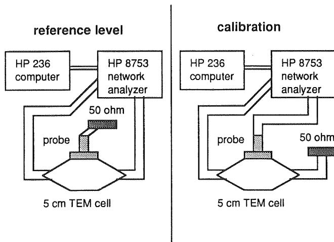
Fig. 8: Probe Calibration
