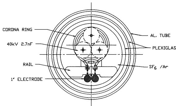
Fig. 4: Cross-sectional View of 600 kV Marx
