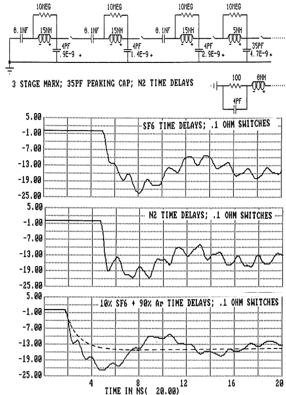
Fig. 3: Computer Simulation of Circuit Model
