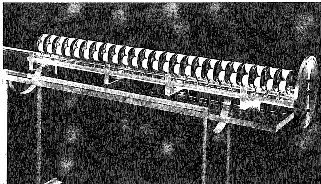
Fig. 5: 24 Stage Assembly
