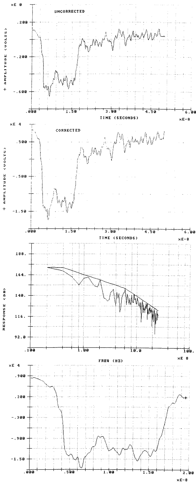
Fig. 10: Time Domain and FFT Results in 10% SF 6 + 90% Ar
