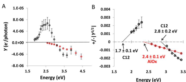
Figure 2. (A) Photocurrent yield spectra for two junctions (Al/AlO x /Cu, red curve, and carbon/C12/Cu, black curve). (B) Corresponding Fowler plots with extrapolated barrier values. C12 data is from a previous report. 44
