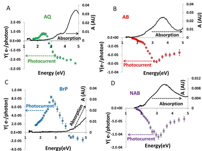
Figure 4. Overlay of photocurrent yield and absorption spectra for four different junctions; black line indicates the optical absorption spectra of the molecular layer corrected for PPF absorbance, and the colored line indicates the measured photocurrent spectrum of a particular molecule (A) AQ, (B) AB, (C) BrP, and (D) NAB.
