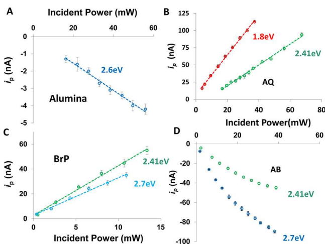
Figure 5. Photocurrent vs light intensity curves for (A) Al/AlO x /Cu, blue curve at 2.6 eV (476 nm); (B) carbon/AQ/Cu at 1.8 eV (688 nm), red curve, and 2.4 eV (516 nm), green curve; (C) carbon/BrP/Cu at 2.4 eV (516 nm), green curve, and 2.7 eV (458 nm), blue curve; (D) carbon/AB/Cu at 2.4 eV (516 nm), green curve, and 2.7 eV (458 nm), blue curve.
