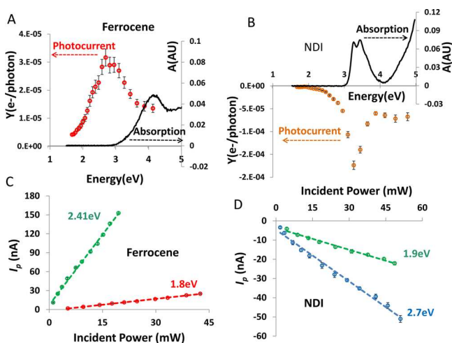
Figure 6. Overlay of photocurrent yield (colored lines) and absorbance spectra (black lines), for (A) Fc and (B) NDI. (C) Photocurrent vs intensity for PPF/Fc/Cu at 2.4 eV (green line), and 1.8 eV (red). (D) Photocurrent vs intensity for PPF/NDI/Cu at 2.7 eV (blue) and 1.9 eV (green).
