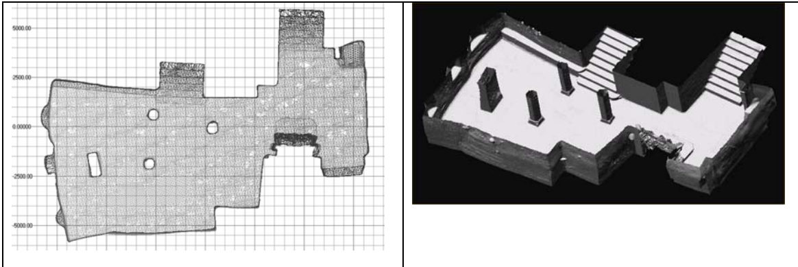
Figure 2. Complete 3D model of the Byzantine Crypt, a) view from outside shown with synthetic shading, b) a particular view of the stairs leading to the Crypt, c) floor plan generated from an orthographic view of the 3D model, d) section of 3D model showing the space inside the crypt.
