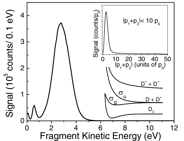
FIG. 1. The main figure shows the measured distribution of correlated D^+ fragments resulting from irradiating D_2 with 3 \times 10^{14} W/cm 2 , circularly polarized light. The upper right figure shows the momentum sum for the two fragments. The pair was considered coincident if the sum of momenta was less than 10p_0 , with p_0 = e^2/\hbar the atomic unit of momentum. The potential energy diagram for D_2 is in the lower right. The laser pulse will singly ionize D_2 , leaving D_2^+ in the \sigma_g state. Shakeup will leave D_2^+ in the excited \sigma_u state, resulting in greater kinetic energy release.
