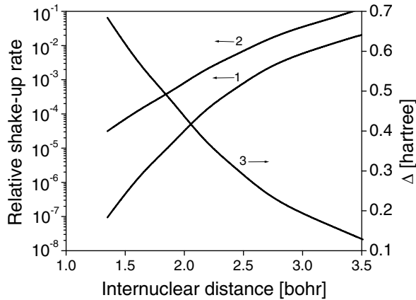
FIG. 3. Relative shakeup rates in D_2 as a function of internuclear distance. Curve 1 (SU1) depicts w_1/w_0 ; see Eq. (1). Curve 2 (SU2) depicts v_1/w_0 ; see Eq. (4). The rates have been averaged over \varphi , the angle between the laser electric field and the molecular axis. Shakeup is calculated at the intensity 8 \times 10^{14} W/cm ^2 . Curve 3 shows \Delta , the energy difference between the ionic \sigma_g and \sigma_u states of D_2^+ .
