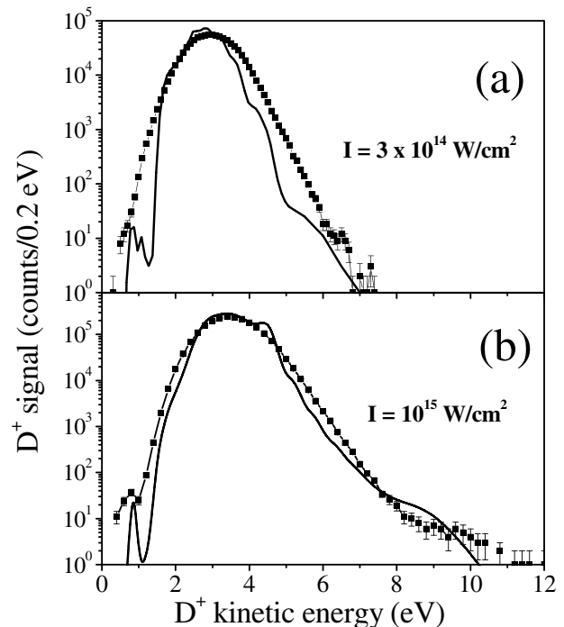
FIG. 2. The dots represent the experimental measurement of kinetic energy release per D_2 fragment, shown with a log scale. The solid curve is the calculation. Two laser intensities are shown. Only for the higher intensity of 10^{15} W/cm 2 is there evidence of shakeup events above 8 eV. The measured branching ratio is 2 \times 10^{-5} .
