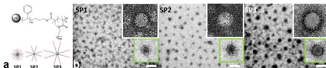
Figure 1. SP2 SP3 Figure 1. Three different star polymers (SPs): a) molecular structure and schematic diagram, b) STEM and TEM (top insets) images. Scale bar = 50 nm.
