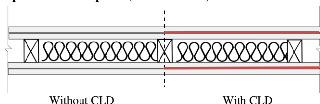
Without CLD With CLD Figure 1 – Wall assemblies viewed from above
