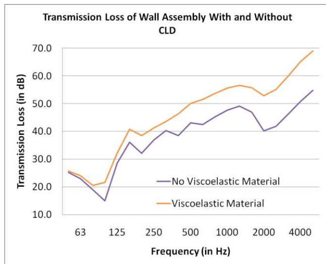
Figure 3 – Measured transmission loss with and without constraint layer damper (CLD).
