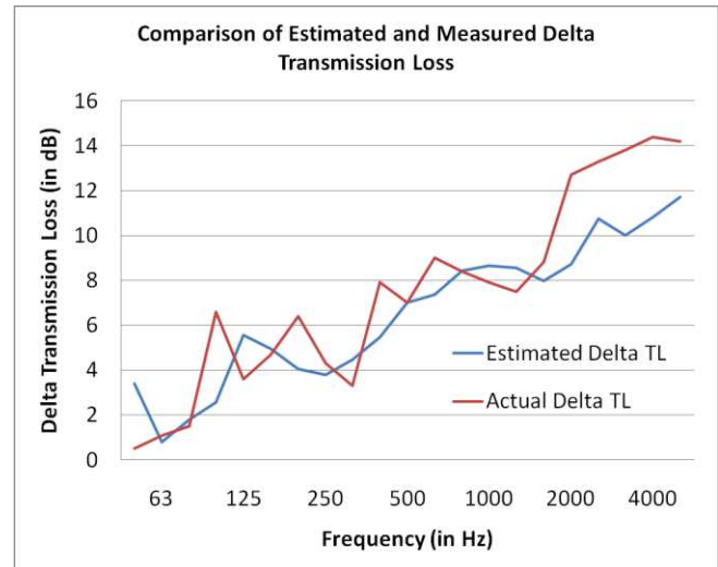
Figure 4 – Comparison of estimated and measured change in transmission loss.
