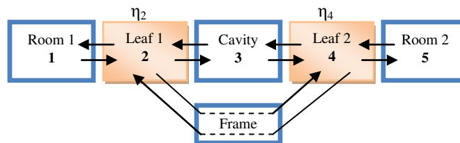
Figure 2 – Simplified SEA model of two rooms separated by a double leaf wall
