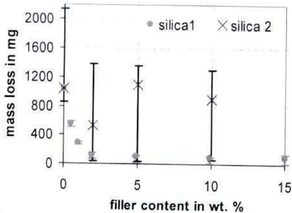
Figure 1. Median, maximum and minimum values of the mass loss occurring during the tracking and erosion test (according to IEC 60587) of a silicone matrix material with two different silica filler materials for three samples each
