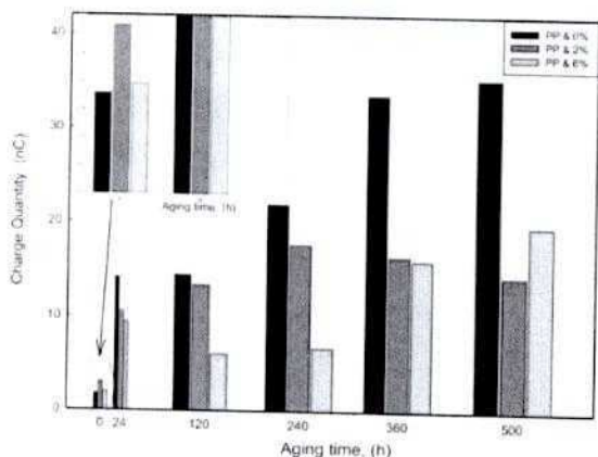
Figure 1. Charge vs. aging time for PNC containing 0, 2 and 6 wt% organoclay [17, 20]
