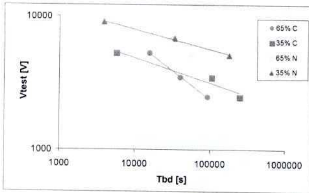
Figure 1. Obtained life curves. C=Conventional Enamel, N=Nanocomposite Enamel
