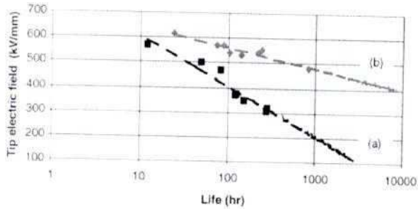
Figure 2. Voltage endurance for 10% loaded epoxy resin loaded with 10% (a) microparticles and (b) nanoparticles of TiO_2 ; after [3].
