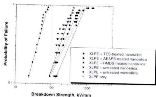
Figure 1. The cumulative probability of breakdown (DC, uniform field) as a function of electrical field for crosslinked polyethylene containing different nanoparticles. TES=Triethoxyvinylsilane, AEAPS=aminopropyltrimethoxysilane, HMDS=hexamethyldisilazane [1].
