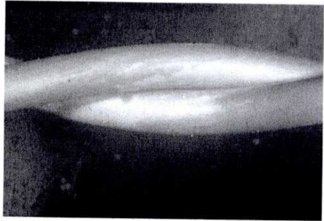
Figure 3. Damaged area: Nanocomposite Enamel, 65% RH, 9000 V
