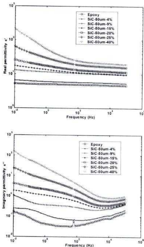
Figure 1. Real (a) and imaginary (b) part of the complex permittivity of epoxy/SiC p - 50 μm composite as function of frequency (from [7]).
