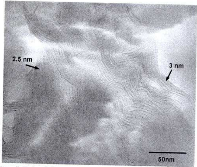
Figure 2. High resolution transmission electron micrographs of nanocomposite materials showing the components having variable size and structure down to the nanometer level.
