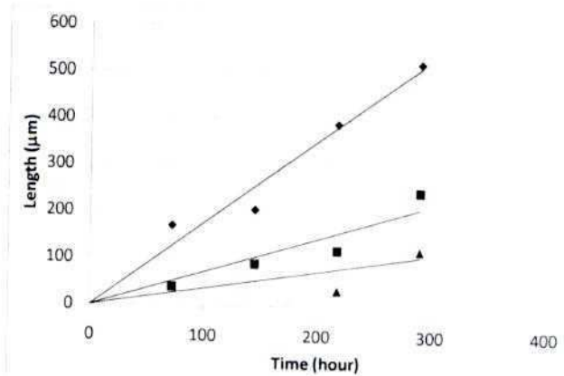
Figure 4. Water tree growth for XLPE- SiO_2 nanocomposite with loadings of 0% ( \bullet ), 5% ( \blacksquare ), and 12.5% ( \blacktriangle ); (after [6]).
