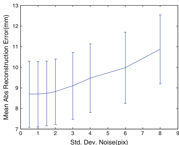
Fig. 5 Influence of an auto-regressive noise added to input silhouettes on the accuracy of the reconstruction body shape
