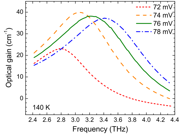
FIG. 10. (Color online) Gain spectra simulated using NEGF model at T=140 K and different biases per module.
