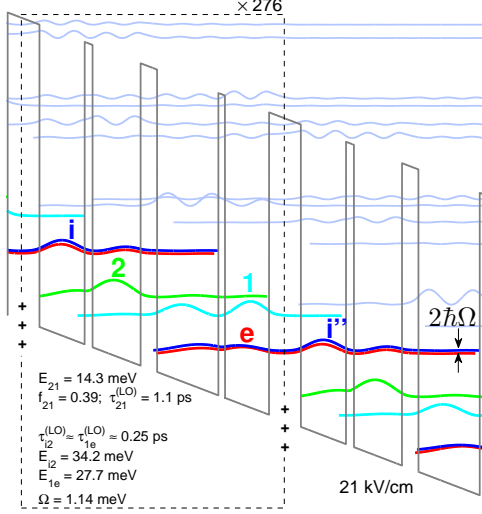
FIG. 2. (Color online) Conduction band diagram and the moduli squared of wavefunctions at 21 kV/cm of the designed THz QCL active region based on “phonon-photon-phonon” scheme. The “+” signs denote the ionized impurities used for doping. The LO-phonon emission assisted scattering times \tau_{lm}^{(LO)} are given for the initial kinetic energy E_{LO} - E_{lm} .
