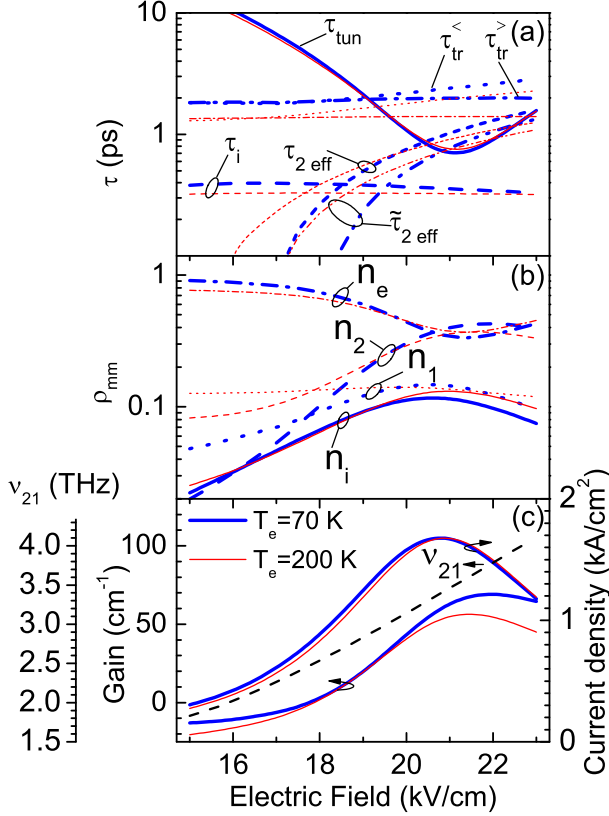
FIG. 3. (Color online) Results of simulations based on the rate equation model performed on the structure proposed in Figure 2. a) Different characteristic times at 20 K (thick lines) and 150 K (thin lines)- 70 K and 200 K for electrons, respectively. As discussed in section II, \tau_{\text{tun}} is tunneling time (solid line); \tau_{\text{tr}}^< (dot line) and \tau_{\text{tr}}^> (dash dot line) are transit times before and after threshold; \tau_i is injection state lifetime (dash line); \tau_{2\text{eff}} is standard effective lifetime of ULS (short dash line); and \tilde{\tau}_{2\text{eff}} is modified effective lifetime (dash dot line). b) Normalized populations of the four states at 20 and 150 K lattice temperatures. c) Current density, lasing frequency and optical gain versus electric field at 20 and 150 K lattice temperatures.
