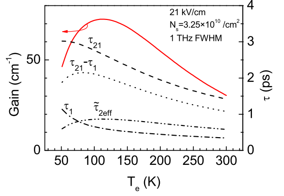
FIG. 4. (Color online) Left axis: peak gain at 21 kV/cm versus the electronic temperature from simulations based on rate equation model. Right axis: intersubband recombination time between lasing states, \tau_{21} , and depopulation time constant, \tau_{1e} , the difference \tau_{21} - \tau_{1e} , and the modified effective lifetime of ULS, \tilde{\tau}_{2\text{eff}} .
