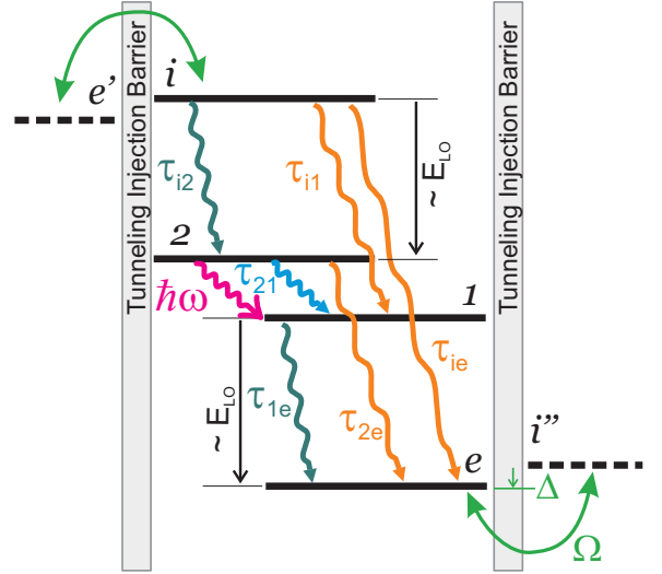
FIG. 1. (Color online) Schematic diagram of a scattering-assisted QCL active region based on a “phonon-photon-phonon” configuration.
