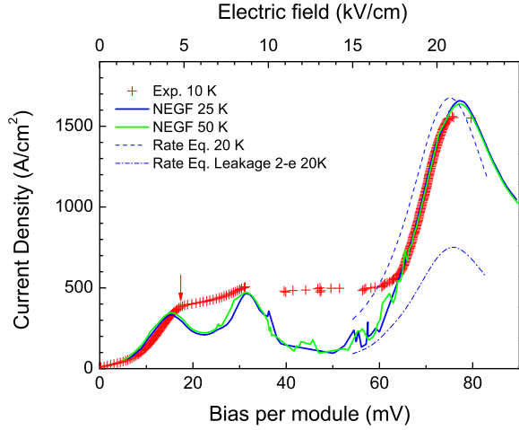
FIG. 9. (Color online) Current density versus voltage bias per period: experimental data (scattered points) at 10 K in pulsed mode and comparison with simulations by nonequilibrium Green's function formalism. The position of the first resonance at \sim 4.8 kV/cm in the experimental data is highlighted by a vertical arrow and is attributed to sequential tunneling from e to 1 and then 2 in three consecutive periods. The NEGF simulation are performed for higher temperatures than the experimental data but the simulated results are weakly temperature sensitive. Moreover, by the end of the current pulses (250 ns) it is well known that the lattice temperature can be several tens of kelvin higher than heat sink. The large fluctuations around 40-60 meV are artifacts of the simulation. The device was driven in current mode which explains why the valley of the second NDR predicted by theory is not observed. The simulated current density by the rate equation model is plotted in dashed line.
