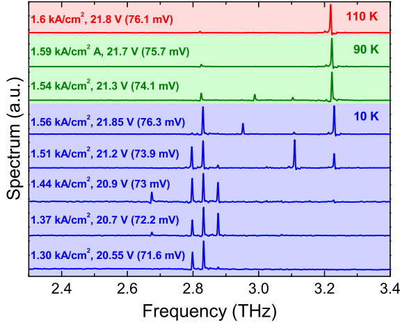
FIG. 7. (Color online) THz spectra recorded for different biases and temperatures. The bias per module is reported between brackets.
