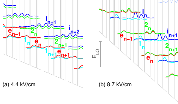
FIG. 6. (Color online) Conduction band diagram and the moduli squared of wavefunctions at a) 4.4 kV/cm and b) 8.7 kV/cm.
