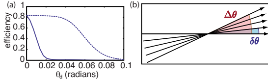
FIG. 6. (Color online) (a) Memory efficiency versus deviation angle \theta_d for an EIT protocol with a wide control beam w_c = 9w_s . The dotted line corresponds to zero phase mismatch, the solid line to \delta\chi = 1 . (b) Angular multiplexing. Different signal fields may be stored with different angles \theta . Provided the difference \delta\theta in angle between adjacent modes is large enough, the modes are “holographically isolated” and may be addressed, and resolved, independently. The largest angle \Delta\theta for which the memory protocol is acceptably efficient sets a limit to the multimode capacity of such a multiplexed memory.
