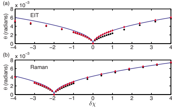
FIG. 3. (Color online) Comparison of numerical results for the optimal angle \theta with the prediction in Eq. (1) (solid line). The filled circles correspond to tight control focusing, with w_c = w_s ; the open diamonds correspond to loose focusing, with w_c = 2w_s . We plot the results for a typical EIT protocol in (a): the signal pulse bandwidth is of order \gamma , the ensemble optical depth is d=30 . In (b) we present equivalent results for a Raman protocol, with the larger optical depth of d=300 . The signal bandwidth is of order 10\gamma and the detuning is \Delta=150\gamma .
