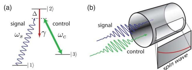
FIG. 1. (Color online) (a) The level structure of the atoms in a typical ensemble memory. (b) A schematic of the storage process, in which an incident signal field is converted to a distributed excitation within the ensemble known as a spin wave.
