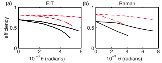
FIG. 5. (Color online) Efficiency versus optimal phase-matching angle. The solid lines correspond to tight control focusing w_c = w_s , the dotted lines to looser focusing, with w_c = 2w_s . Each line has two “branches”: the upper branch is achieved for positive momentum mismatch, the lower for negative momentum mismatch. The results for the EIT protocol are plotted in (a); those for the Raman protocol in (b).
