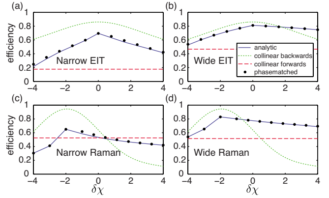
FIG. 4. (Color online) Memory efficiencies versus the phase mismatch \delta\chi . (a) and (b) contain the results for the EIT protocol, with tight and loose focusing, respectively. (c) and (d) report the results for the Raman protocol for tight and loose focusing. The solid lines represent the efficiencies achieved if the angles predicted by Eq. (1) are used. The filled circles are the best efficiencies achievable. The dotted lines delimit the optimal efficiency attainable using collinear backwards retrieval, calculated using the one-dimensional theory described in Appendix A. The dashed straight lines denote the efficiencies achieved using collinear forwards retrieval.
