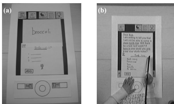
Figure 2: Paper Prototype Showing (a) Word Look-Up Facility and (b) Word Correction Facility
