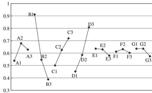
Fig. 9. Design variable sensitivities.
