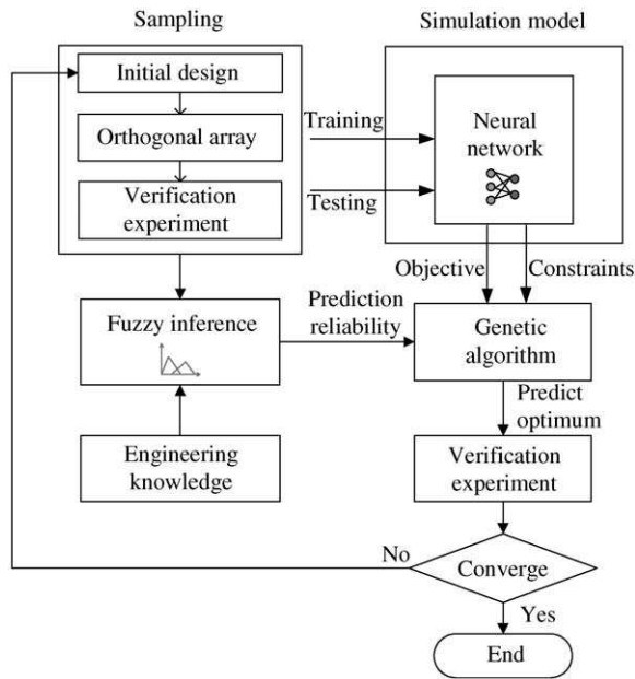
Fig. 3. The optimization flowchart of FUNTGA method.
