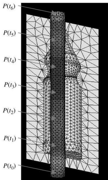
Fig. 2. Programming points of parison extrusion.
