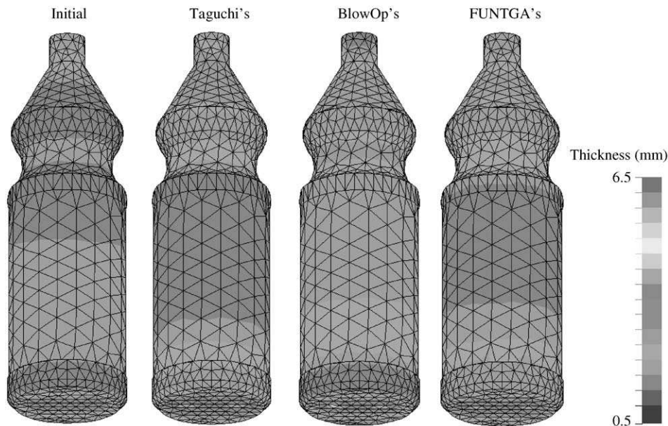
Fig. 11. The comparison of thickness distribution.
