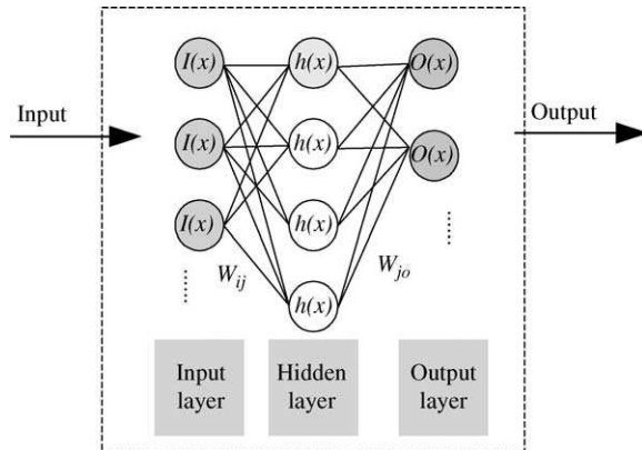
Fig. 5. Back-propagation network.
