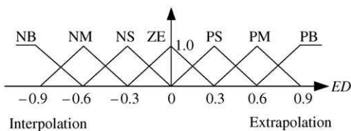
Fig. 7. The membership functions of the conditioned variables.
