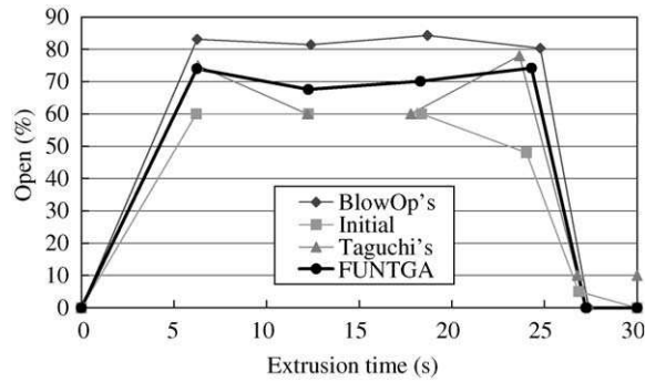
Fig. 10. The optimum designs using various methods.
