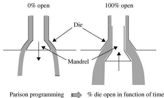
Fig. 1. The parison thickness control using the die gap programming (VWDS).
