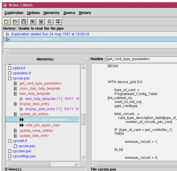
Figure 6: The main window of the tksee tool.
